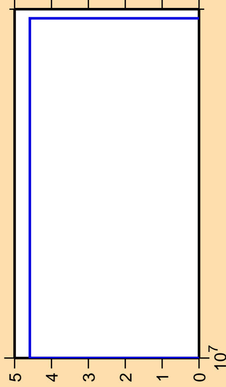
\Delta\sigma/\sigma vs. E for ^{235}\text{Pu}(n,n_2)
