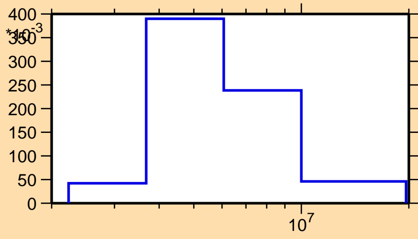
\sigma vs. E for ^{235}\text{Pu}(n,\text{inel.})
