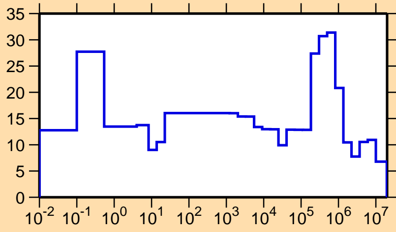
\Delta\sigma/\sigma vs. E for ^{235}\text{Pu}(n,el.)
