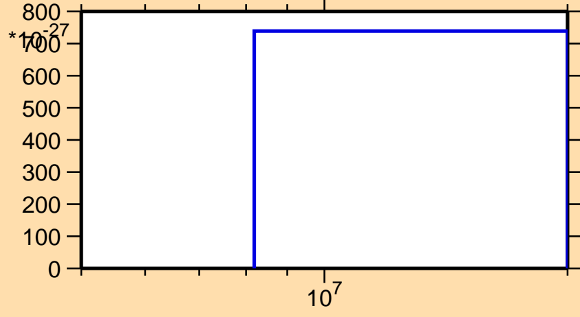
\sigma vs. E for ^{235}\text{Pu}(\text{mt } 42)
