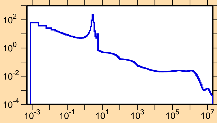
\sigma vs. E for ^{236}\text{Pu}(n,\gamma)
