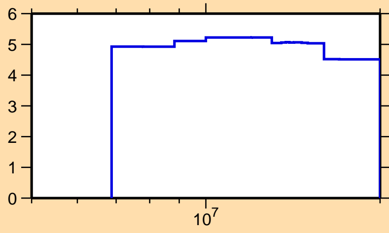
\Delta\sigma/\sigma vs. E for ^{236}\text{Pu}(n,\text{nonel.})
