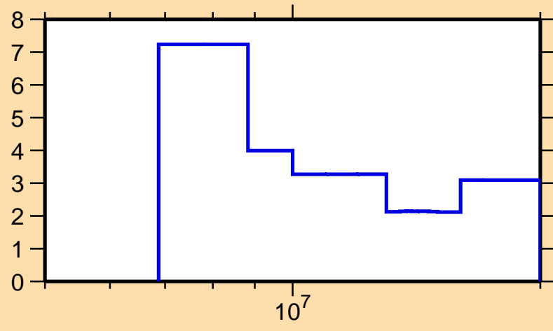
\Delta\sigma/\sigma vs. E for ^{236}\text{Pu}(n,\text{tot.})
