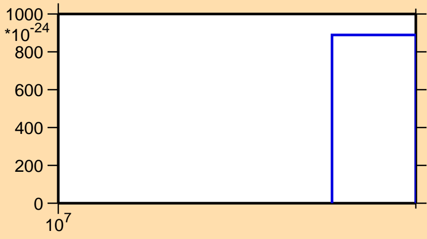
\sigma vs. E for ^{236}\text{Pu} (mt 42)
