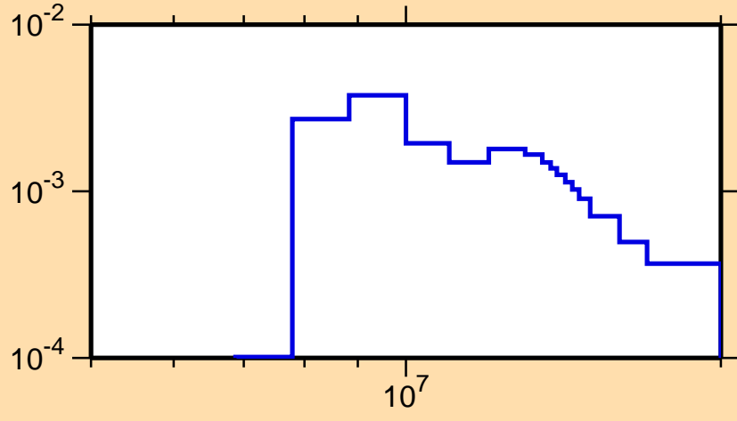
\sigma vs. E for ^{236}\text{Pu}(n,2n)
