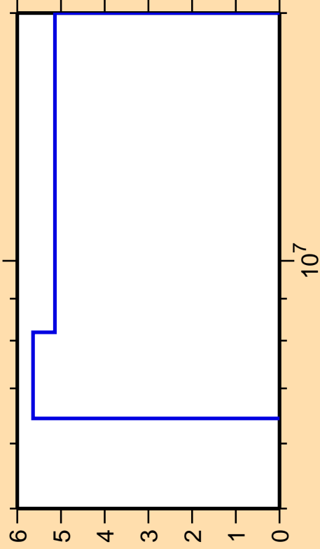
\Delta\sigma/\sigma vs. E for ^{236}\text{Pu}(n,f)
