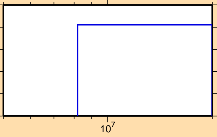
\sigma vs. E for ^{236}\text{Pu}(n,\text{He3})
