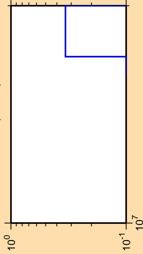
\Delta\sigma/\sigma vs. E for ^{237}\text{Pu} (mt 34)
