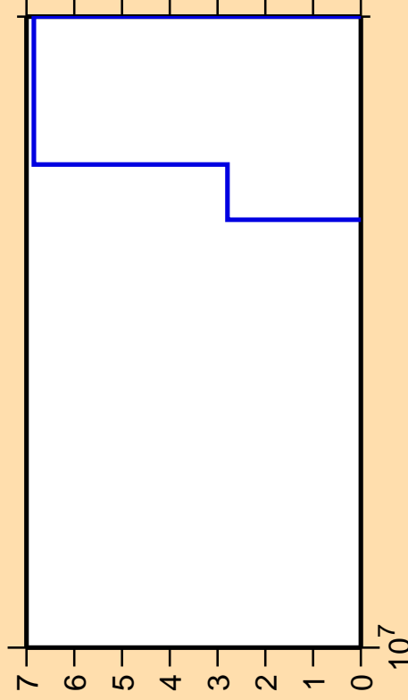
\Delta\sigma/\sigma vs. E for ^{237}\text{Pu}(n,p\alpha)
