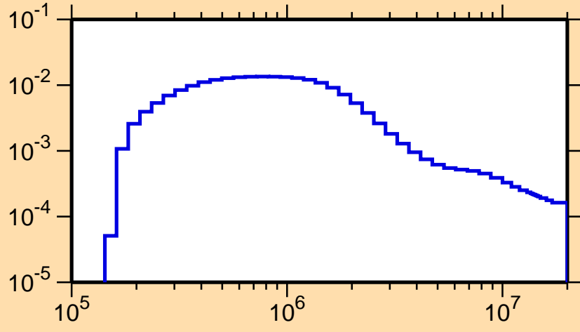
\sigma vs. E for ^{237}\text{Pu}(n,n_4)
