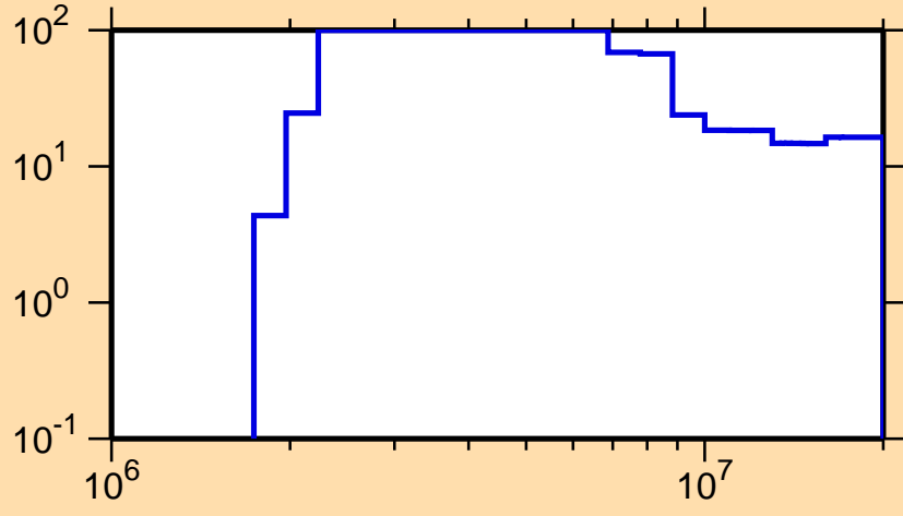
\Delta\sigma/\sigma vs. E for ^{237}\text{Pu}(n,p)
