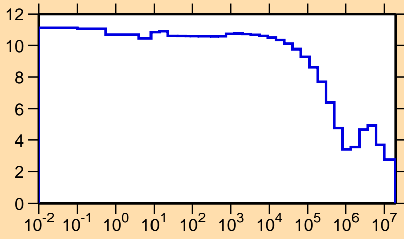
\sigma vs. E for ^{237}\text{Pu}(n,\text{el.})
