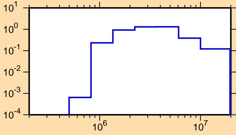
\sigma vs. E for ^{237}\text{Pu}(n,n\text{cont.})
