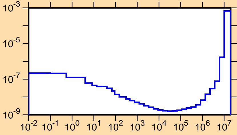
\sigma vs. E for ^{237}\text{Pu}(n,\alpha)
