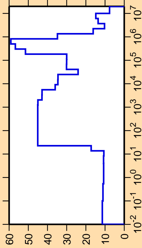
\Delta\sigma/\sigma vs. E for ^{237}\text{Pu}(n,\text{el.})
