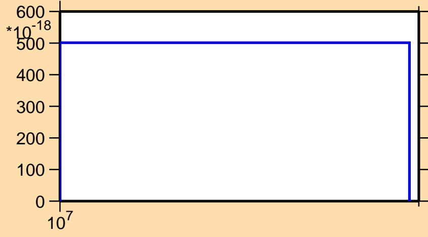
\sigma vs. E for ^{237}\text{Pu} (mt 34)
