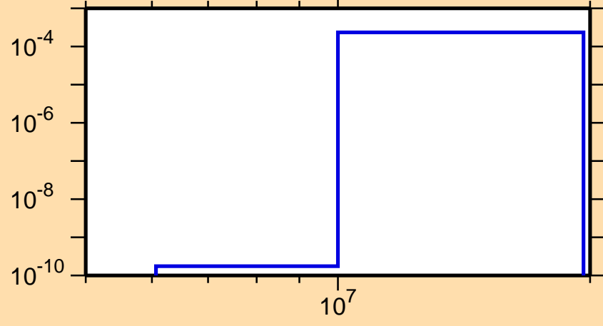
\sigma vs. E for ^{237}\text{Pu}(n,d)
