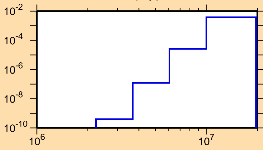
\sigma vs. E for ^{237}\text{Pu}(n,p)
