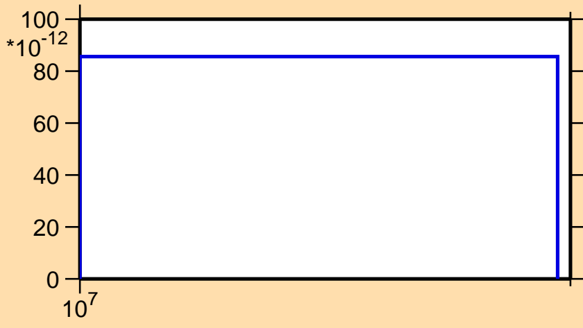
\sigma vs. E for ^{237}\text{Pu}(n,nt)
