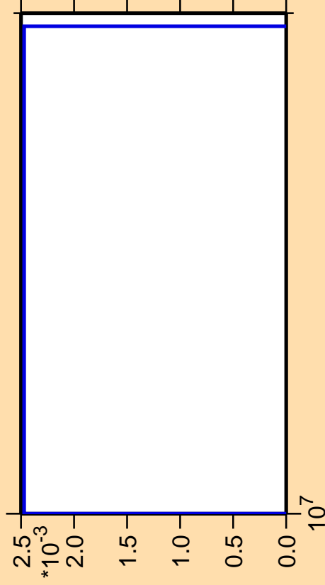
\Delta\sigma/\sigma vs. E for ^{237}\text{Pu} (mt 34)
