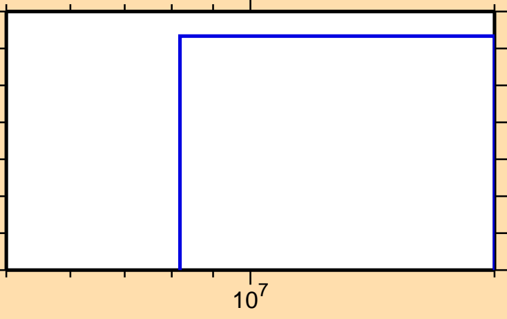
\sigma vs. E for ^{237}\text{Pu}(n,2n\alpha)
