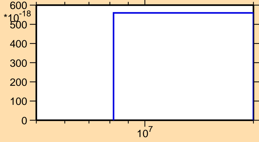
\sigma vs. E for ^{237}\text{Pu}(\text{mt } 34)
