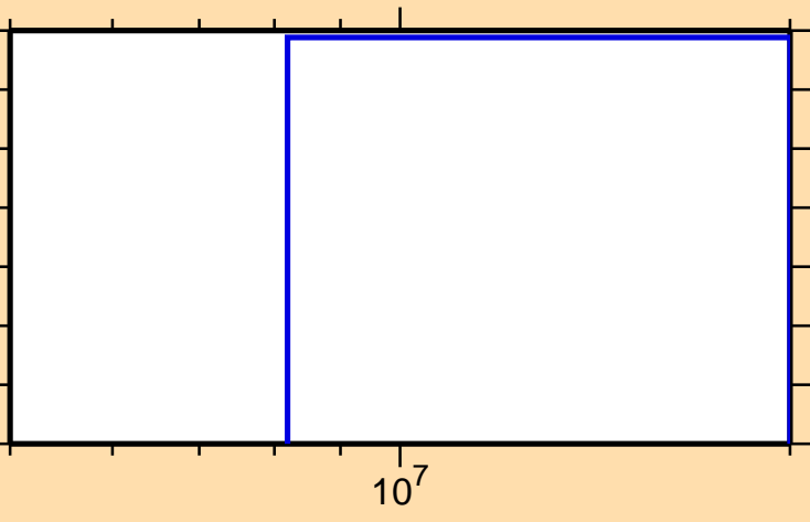
\sigma vs. E for ^{237}\text{Pu}(n,np)
