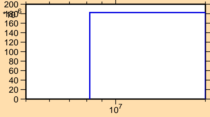
\sigma vs. E for ^{237}\text{Pu}(n,3n)
