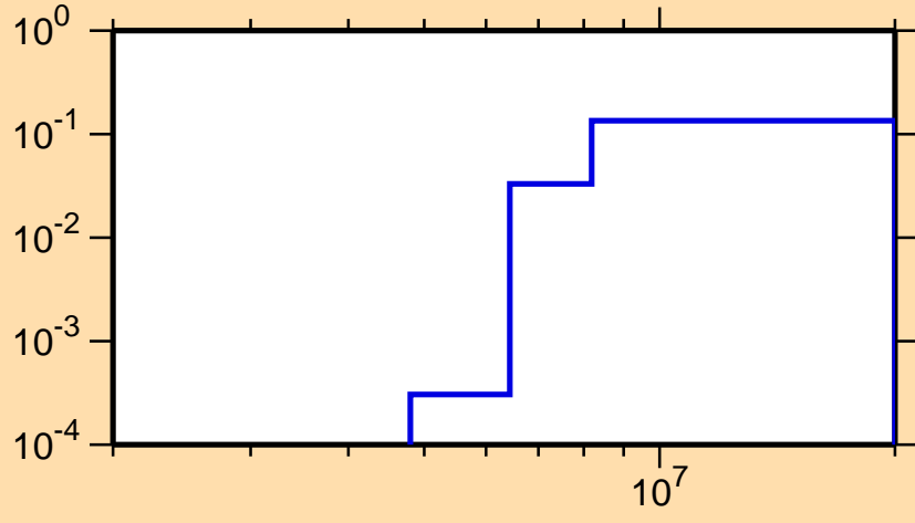
\sigma vs. E for ^{237}\text{Pu}(n,2n)
