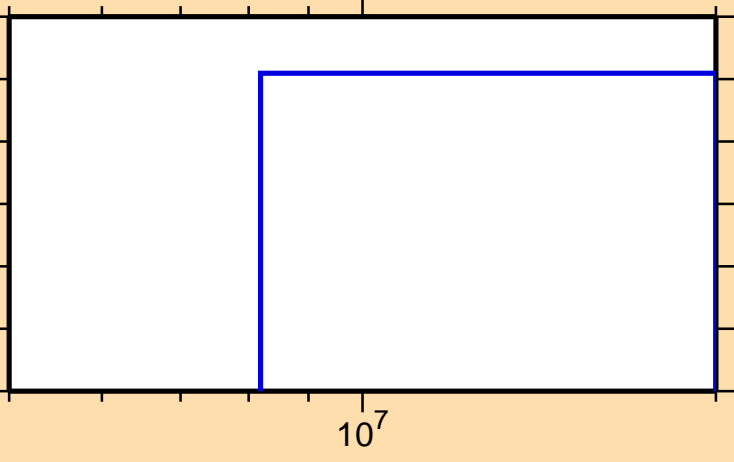
\sigma vs. E for ^{237}\text{Pu}(n,\text{nd})
