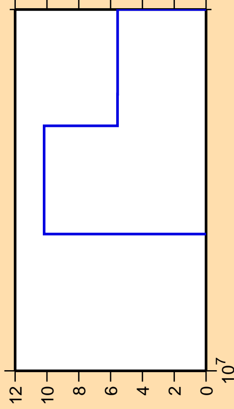
\Delta\sigma/\sigma vs. E for ^{241}\text{Pu}(n,2n\alpha)
