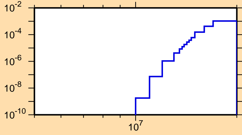
\sigma vs. E for ^{241}\text{Pu}(n,d)
