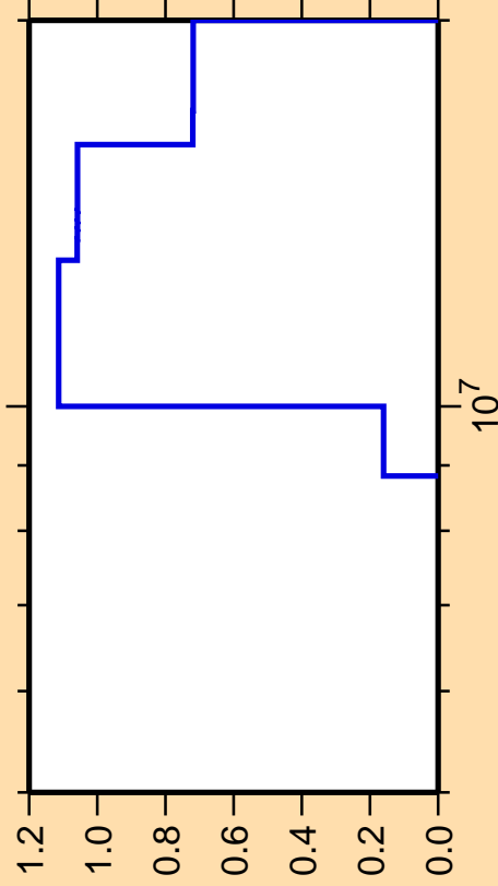
\Delta\sigma/\sigma vs. E for ^{241}\text{Pu}(n,d)
