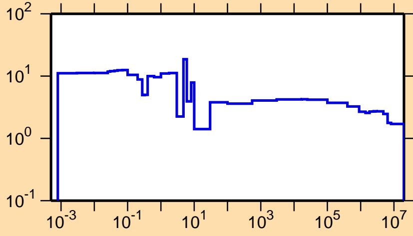
\Delta\sigma/\sigma vs. E for ^{241}\text{Pu}(n,tot.)
