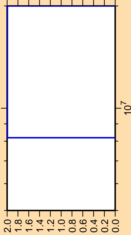
\Delta\sigma/\sigma vs. E for ^{241}\text{Pu}(n,nt)
