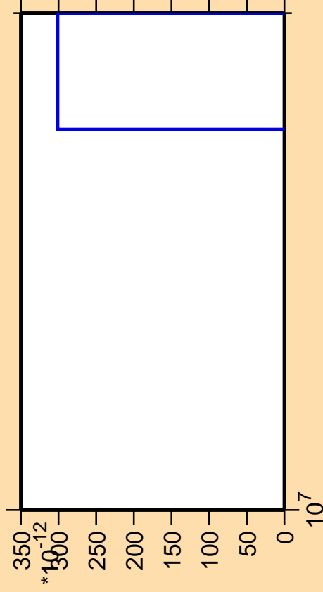
\Delta\sigma/\sigma vs. E for ^{244}\text{Pu}(\text{mt } 42)
