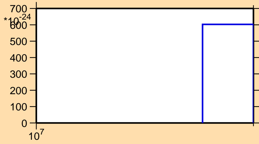
\sigma vs. E for ^{244}\text{Pu}(\text{mt } 42)
