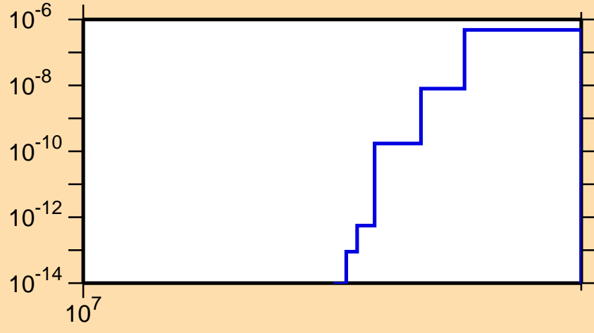
\sigma vs. E for ^{246}\text{Pu}(n,nd)
