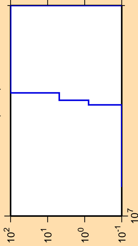
\Delta\sigma/\sigma vs. E for ^{246}\text{Pu}(n,nd)
