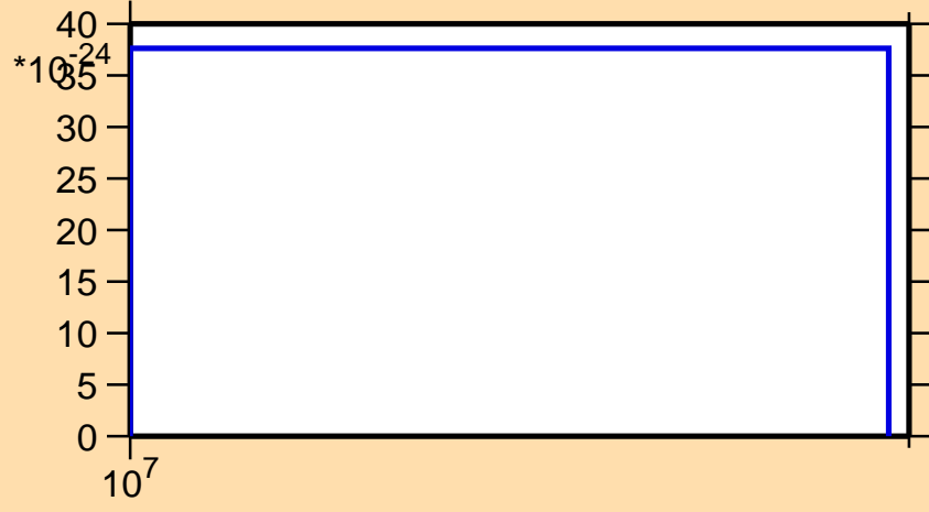
\sigma vs. E for ^{246}\text{Pu} (mt 42)
