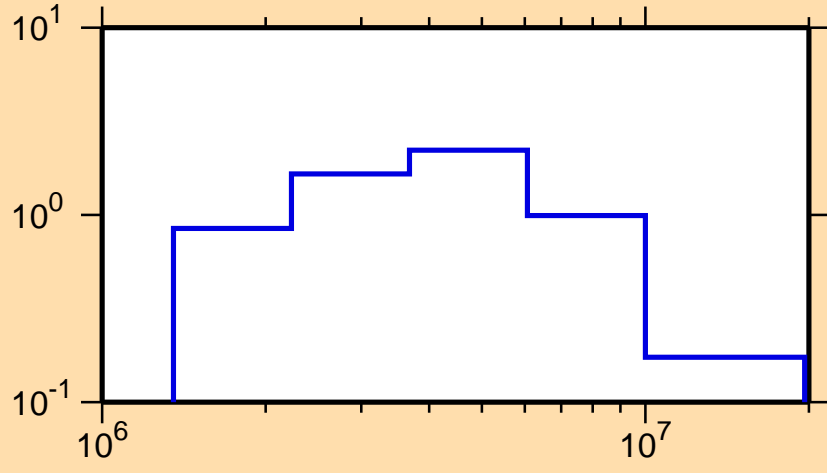
\sigma vs. E for ^{246}\text{Pu}(n,n\text{cont.})
