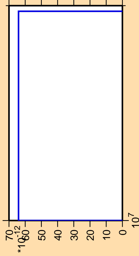
\Delta\sigma/\sigma vs. E for ^{246}\text{Pu} (mt 42)
