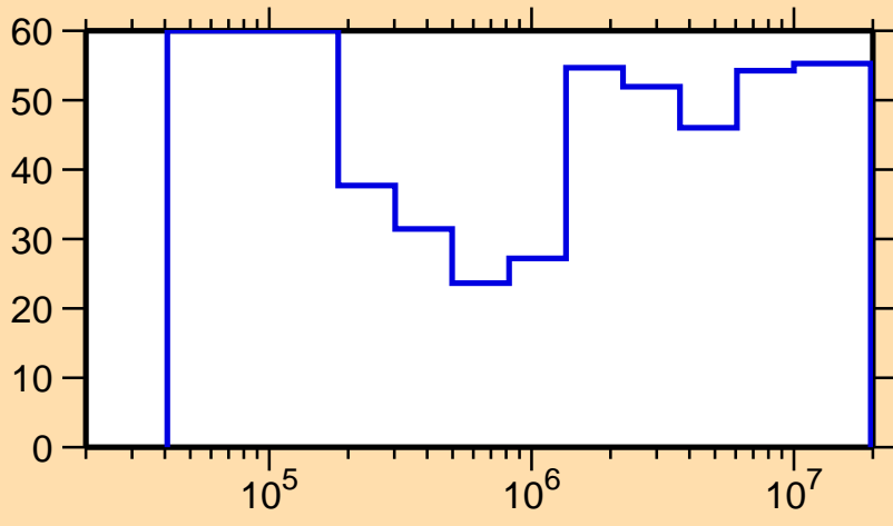
\Delta\sigma/\sigma vs. E for ^{246}\text{Pu}(n,n_1)
