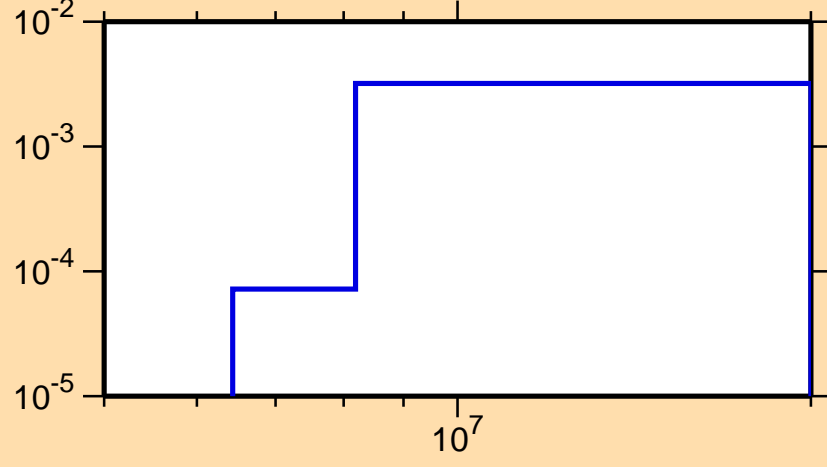
\sigma vs. E for ^{246}\text{Pu}(n,n\alpha)
