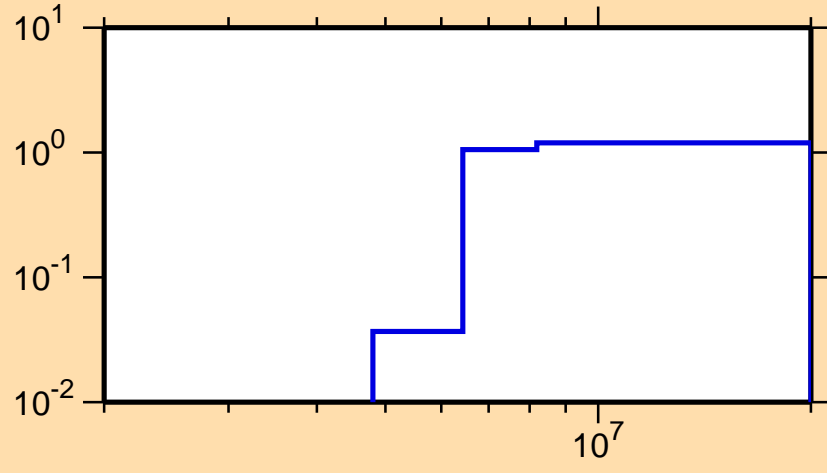
\sigma vs. E for ^{246}\text{Pu}(n,2n)
