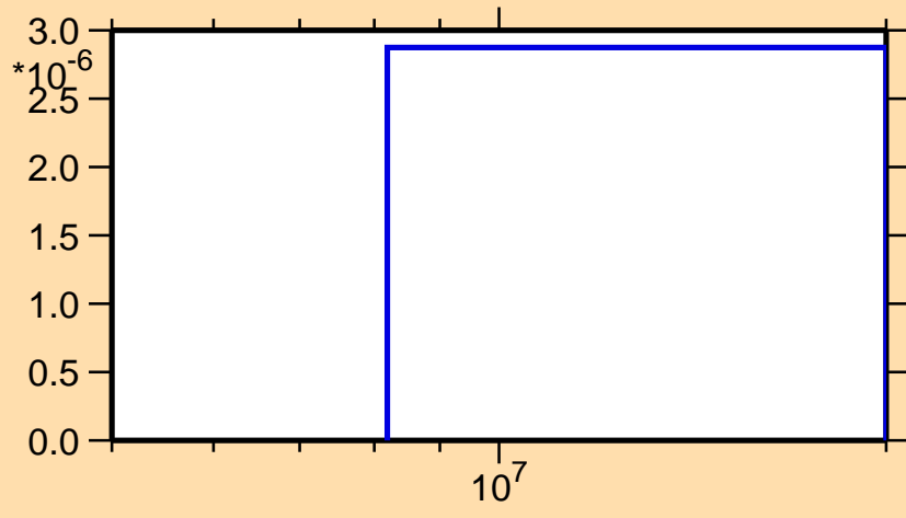
\sigma vs. E for ^{246}\text{Pu}(n,np)
