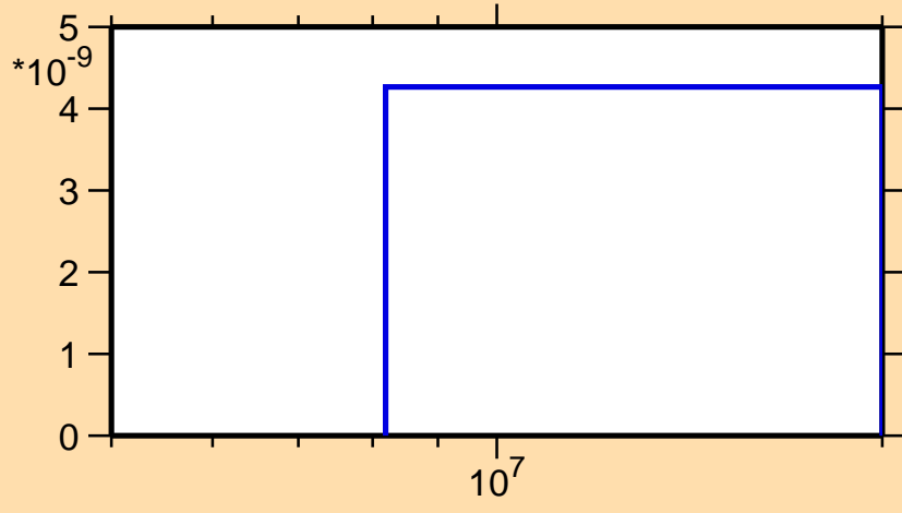
\sigma vs. E for ^{246}\text{Pu}(n,\text{nd})
