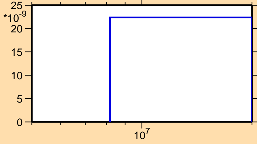
\sigma vs. E for ^{246}\text{Pu}(n,2n\alpha)
