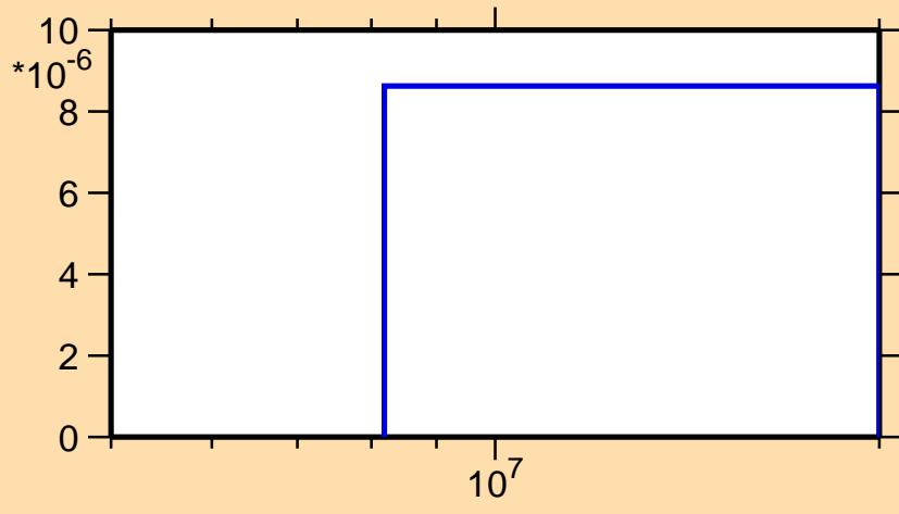
\sigma vs. E for ^{246}\text{Pu}(n,d)
