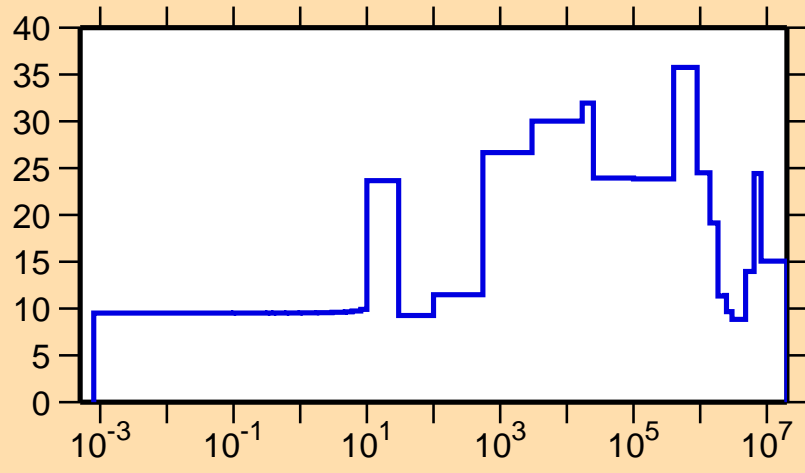
\Delta\sigma/\sigma vs. E for ^{246}\text{Pu}(n,el.)
