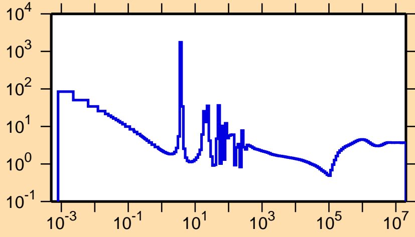
\sigma vs. E for ^{247}\text{Pu}(n,\text{nonel.})
