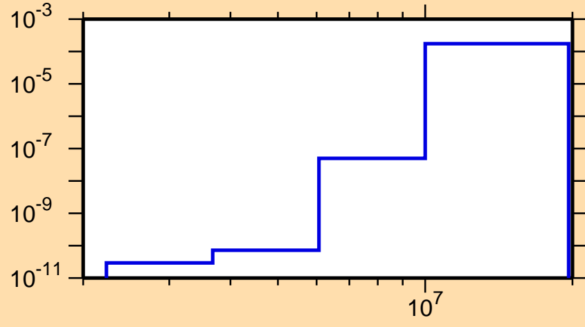
\sigma vs. E for ^{247}\text{Pu}(n,\alpha)
