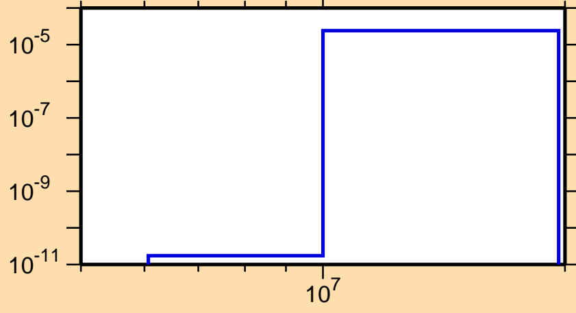
\sigma vs. E for ^{247}\text{Pu}(n,n\alpha)
