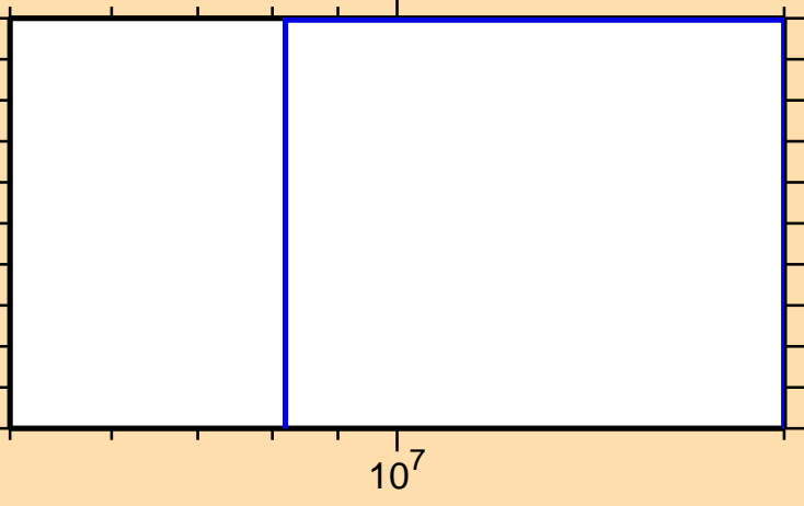
\sigma vs. E for ^{247}\text{Pu}(n,d)
