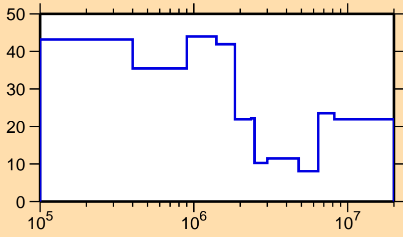
\Delta\sigma/\sigma vs. E for ^{247}\text{Pu}(n,\text{el.})
