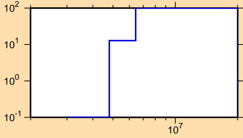
\Delta\sigma/\sigma vs. E for ^{247}\text{Pu}(n,p)
