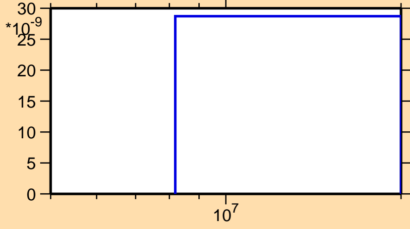
\sigma vs. E for ^{247}\text{Pu}(n,2n\alpha)
