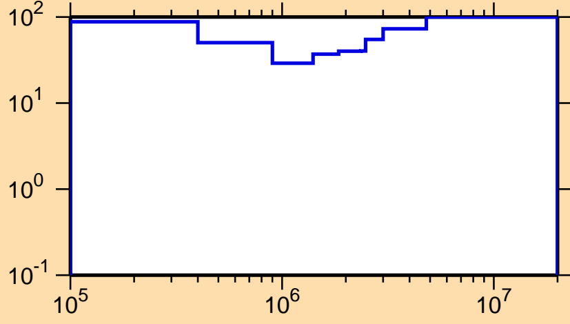
\Delta\sigma/\sigma vs. E for ^{247}\text{Pu}(n,\text{inel.})
