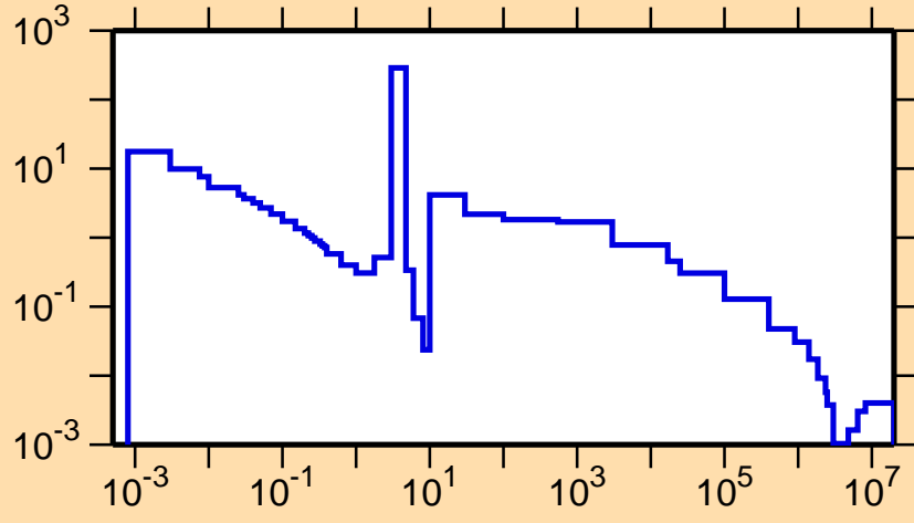
\sigma vs. E for ^{247}\text{Pu}(n,\gamma)
