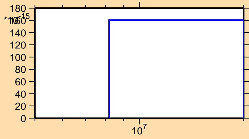
\sigma vs. E for ^{247}\text{Pu}(n,3n\alpha)
