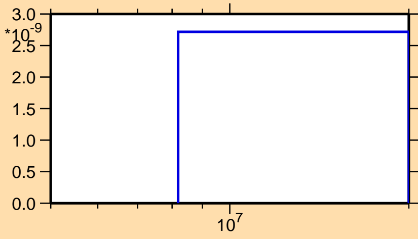
\sigma vs. E for ^{247}\text{Pu}(n,\text{nd})
