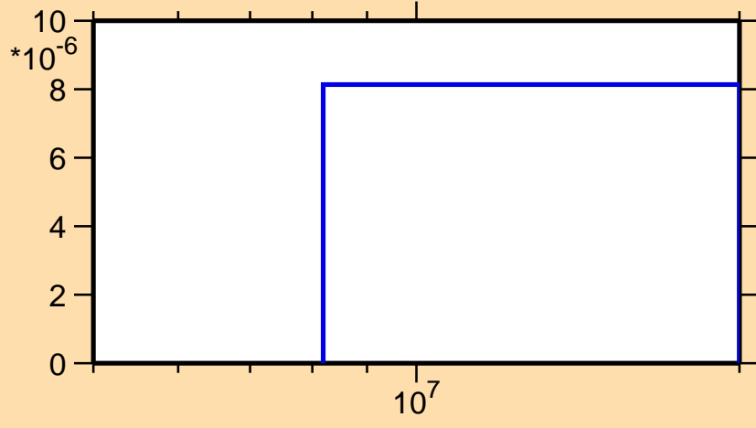
\sigma vs. E for ^{247}\text{Pu}(n,t)
