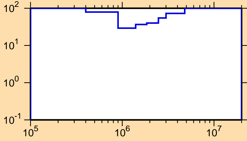
\Delta\sigma/\sigma vs. E for ^{247}\text{Pu}(n,n\text{cont.})
