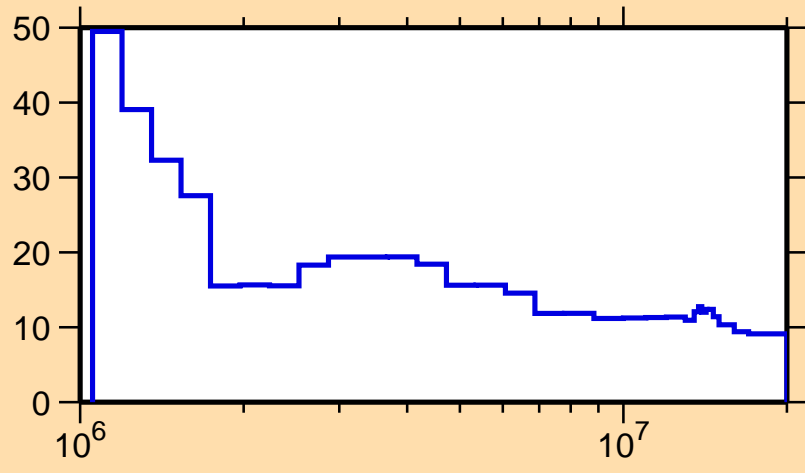
\Delta\sigma/\sigma vs. E for ^{207}\text{Ra}(n,\text{nonel.})
