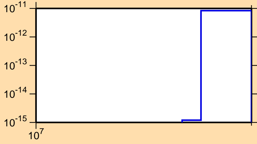
\sigma vs. E for ^{207}\text{Ra}(n,nt)
