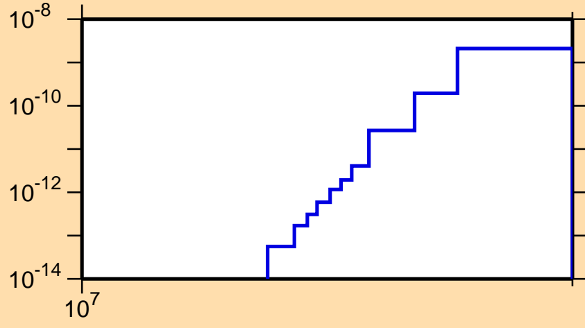
\sigma vs. E for ^{207}\text{Ra}(\text{mt } 34)
