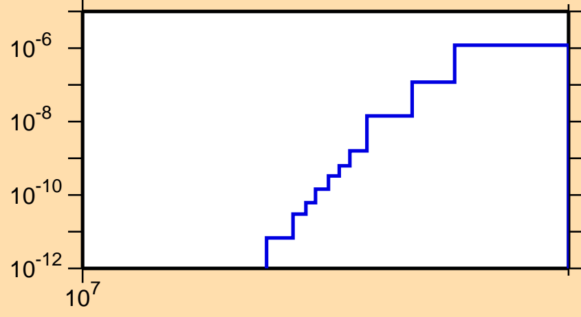
\sigma vs. E for ^{207}\text{Ra}(n,\text{nd})
