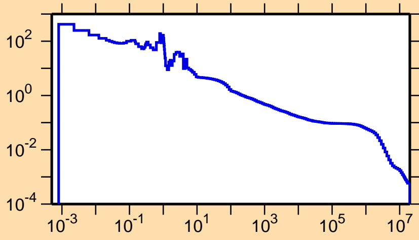
\sigma vs. E for ^{207}\text{Ra}(n,\gamma)
