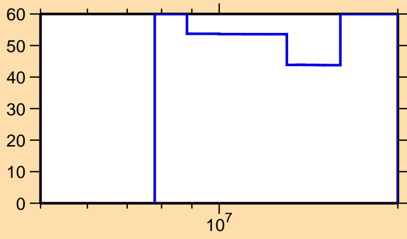
\Delta\sigma/\sigma vs. E for ^{207}\text{Ra}(n,2n)
