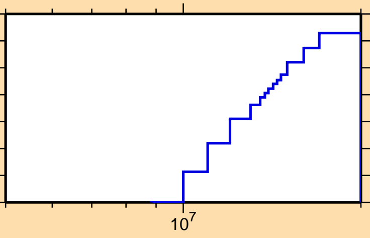
\sigma vs. E for ^{207}\text{Ra}(\text{mt117})
