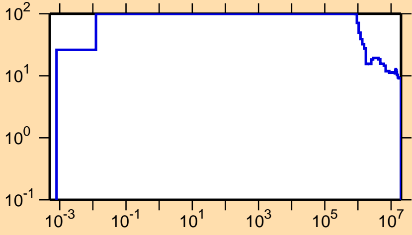
\Delta\sigma/\sigma vs. E for ^{207}\text{Ra}(n,\text{nonel.})
