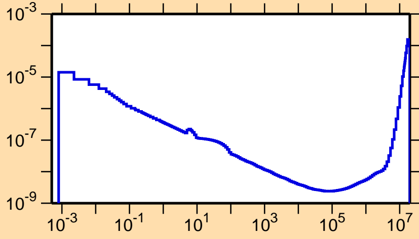
\sigma vs. E for ^{207}\text{Ra}(n,p\alpha)
