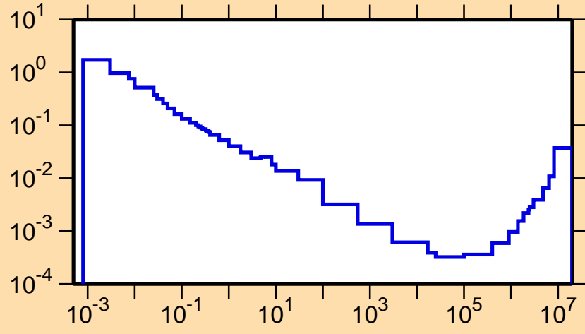
\sigma vs. E for ^{207}\text{Ra}(n,p)
