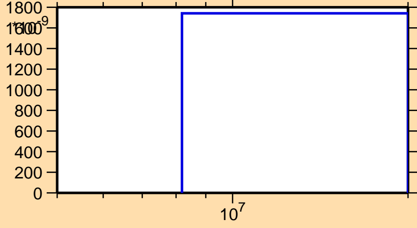
\sigma vs. E for ^{207}\text{Ra}(n,2n\alpha)
