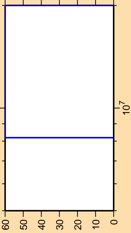
\Delta\sigma/\sigma vs. E for ^{207}\text{Ra}(n,\text{pd})
