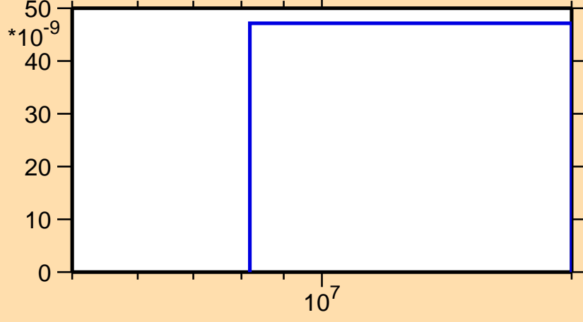
\sigma vs. E for ^{207}\text{Ra}(n,2np)
