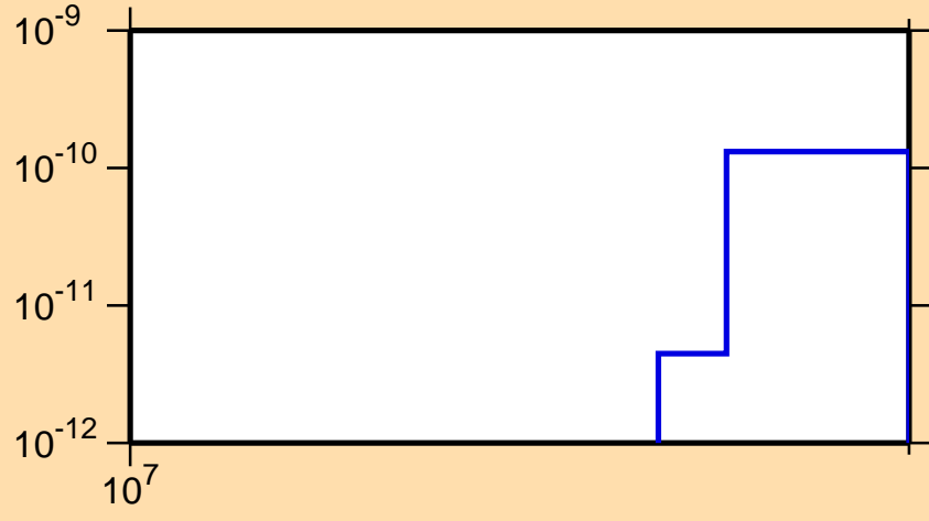
\sigma vs. E for ^{208}\text{Ra} (mt 34)
