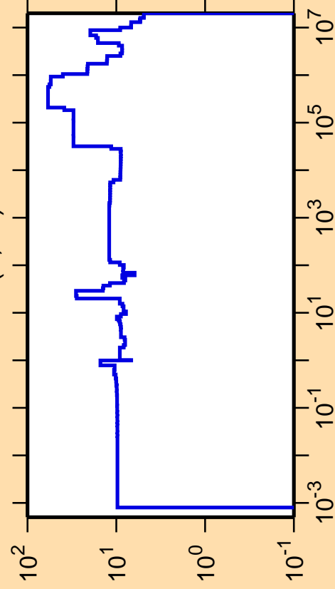
\Delta\sigma/\sigma vs. E for ^{208}\text{Ra}(n,\text{el.})
