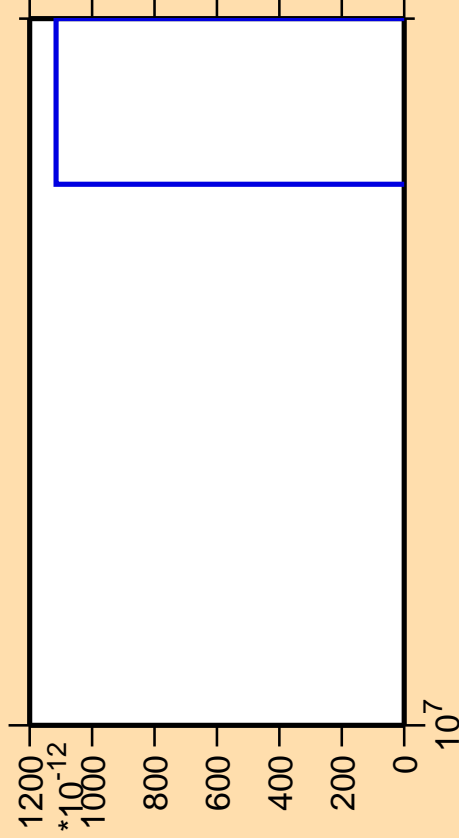
\Delta\sigma/\sigma vs. E for ^{208}\text{Ra} (mt 11)
