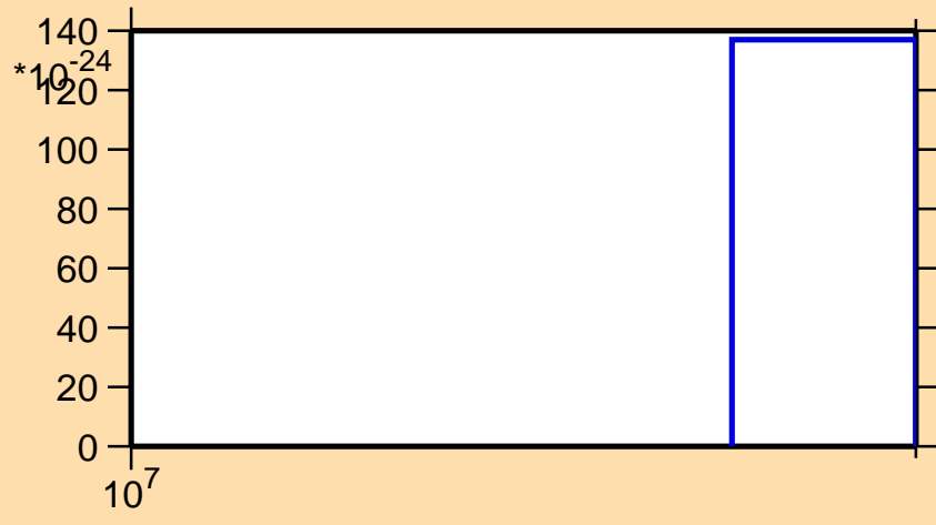
\sigma vs. E for ^{208}\text{Ra} (mt 11)
