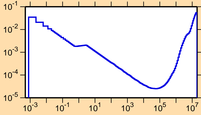
\sigma vs. E for ^{208}\text{Ra}(n,p)
