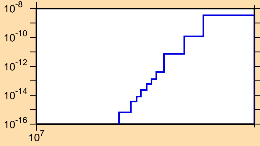
\sigma vs. E for ^{208}\text{Ra}(n,\text{pt})
