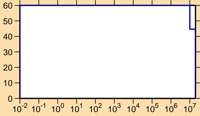
\Delta\sigma/\sigma vs. E for ^{208}\text{Ra}(n,p)
