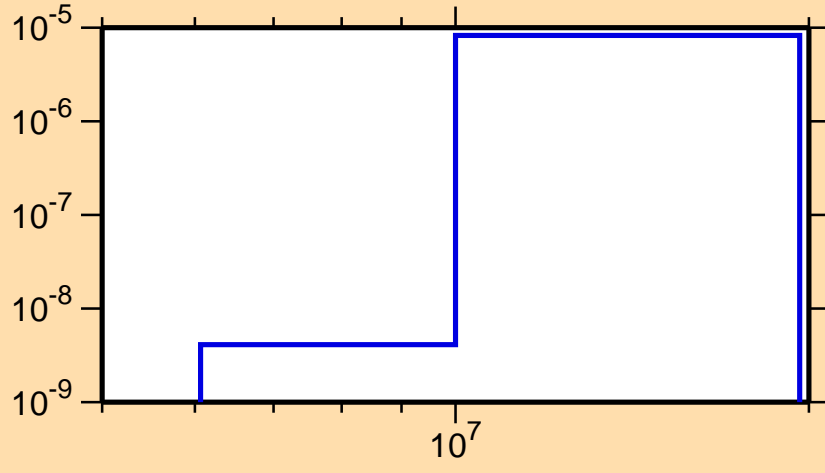
\sigma vs. E for ^{208}\text{Ra} (mt 45)
