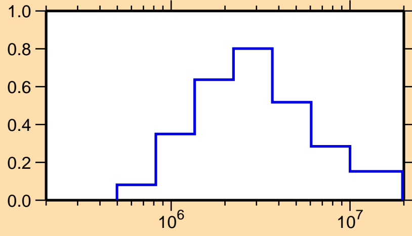
\sigma vs. E for ^{208}\text{Ra}(n,n_1)
