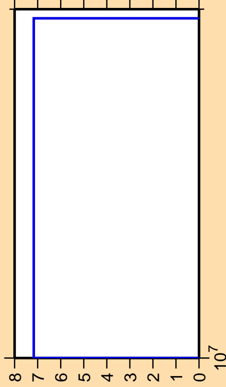
\Delta\sigma/\sigma vs. E for ^{208}\text{Ra}(n,nt)
