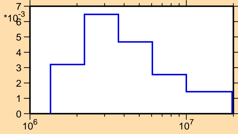
\sigma vs. E for ^{208}\text{Ra}(n,n_3)
