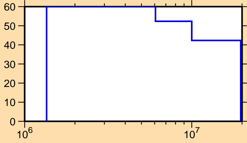
\Delta\sigma/\sigma vs. E for ^{208}\text{Ra}(n,n\text{cont.})
