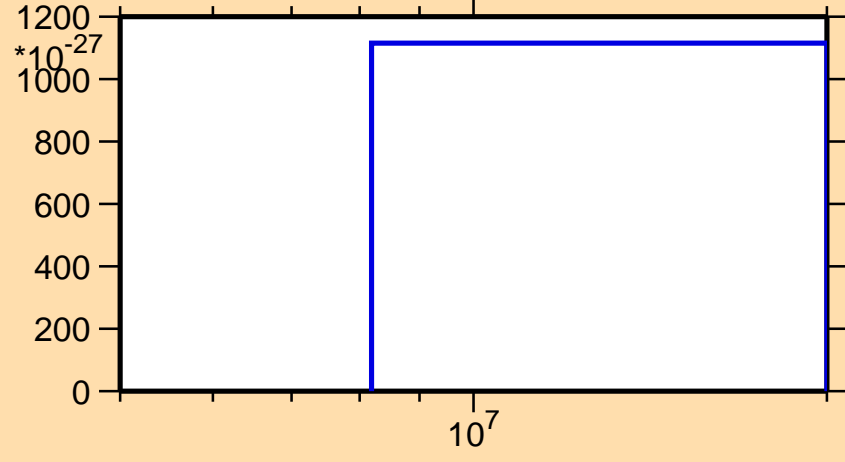
\sigma vs. E for ^{208}\text{Ra} (mt 11)
