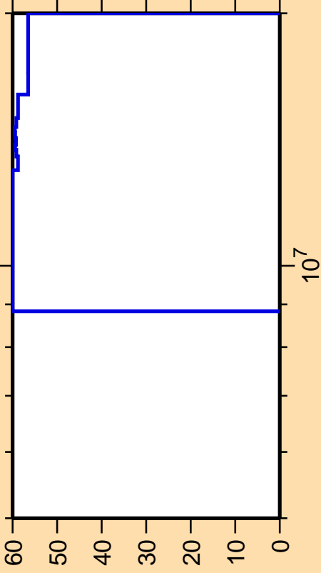
\Delta\sigma/\sigma vs. E for ^{210}\text{Ra}(n,n\text{cont.})
