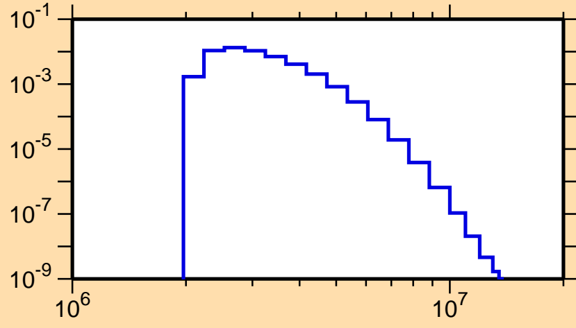
\sigma vs. E for ^{210}\text{Ra}(n,n_4)
