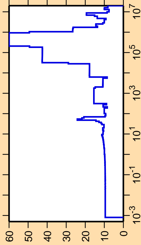
\Delta\sigma/\sigma vs. E for ^{210}\text{Ra}(n,\text{el.})
