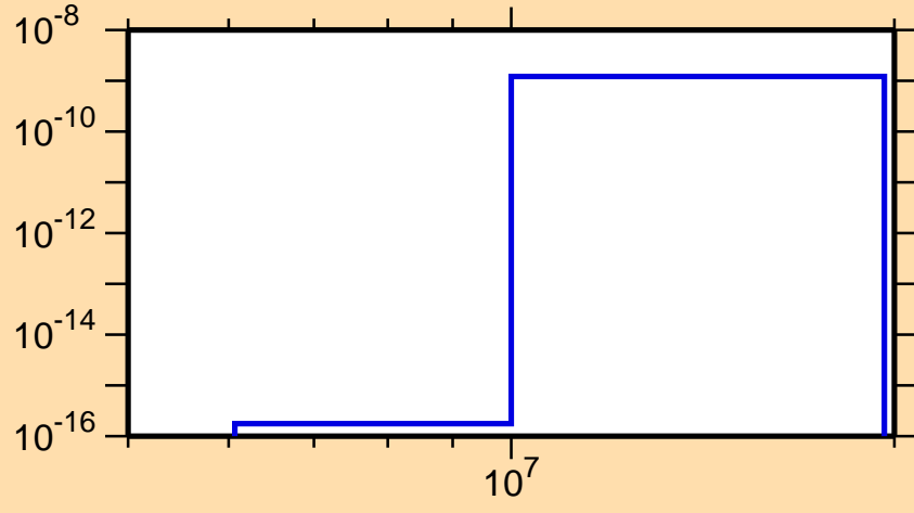
\sigma vs. E for ^{210}\text{Ra}(\text{mt117})
