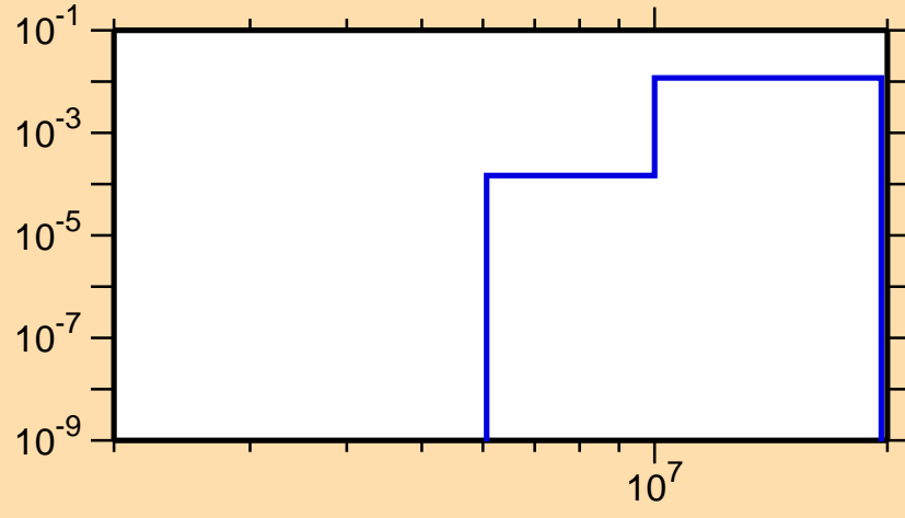
\sigma vs. E for ^{210}\text{Ra}(n,np)
