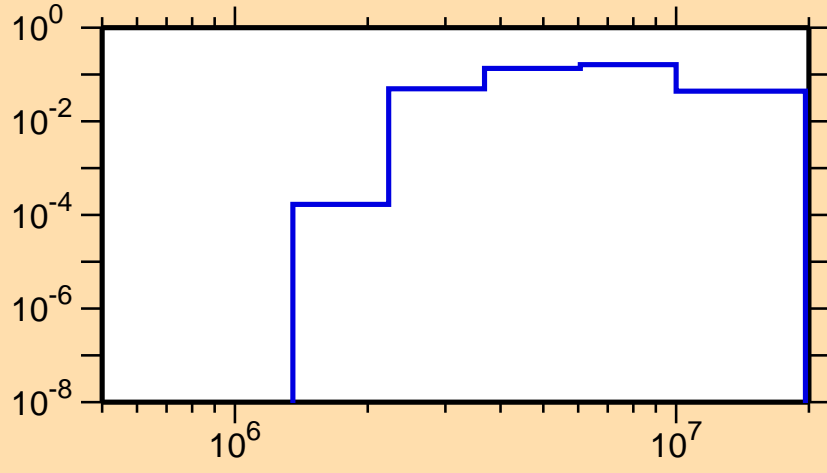
\sigma vs. E for ^{210}\text{Ra}(n,n\alpha)
