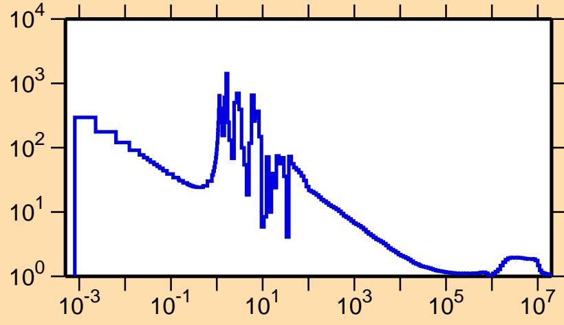
\sigma vs. E for ^{211}\text{Ra}(n,\text{nonel.})
