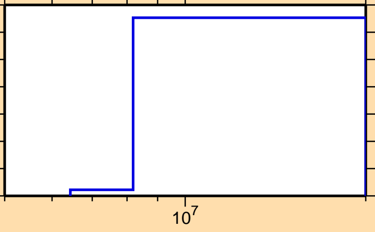
\sigma vs. E for ^{211}\text{Ra}(n,\text{He3})
