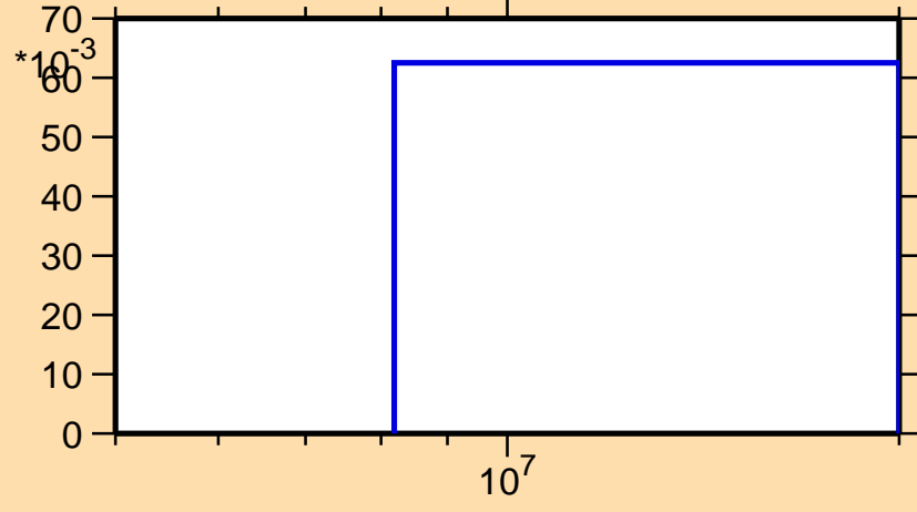
\sigma vs. E for ^{211}\text{Ra}(n,2n\alpha)
