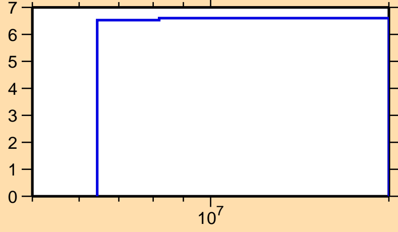
\Delta\sigma/\sigma vs. E for ^{211}\text{Ra}(n,\text{nonel.})
