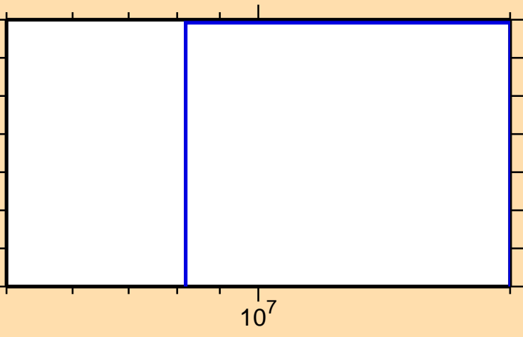
\sigma vs. E for ^{211}\text{Ra}(n,\text{pt})
