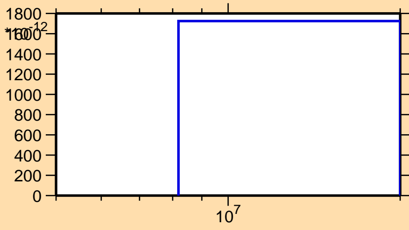
\sigma vs. E for ^{211}\text{Ra}(n,\text{pd})
