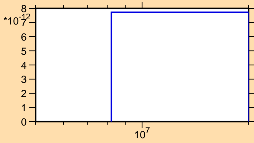
\sigma vs. E for ^{211}\text{Ra}(\text{mt } 34)
