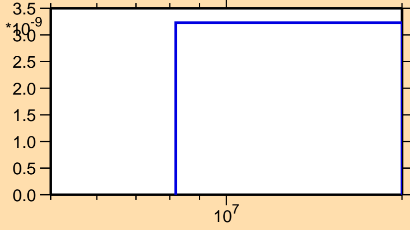
\sigma vs. E for ^{211}\text{Ra}(\text{mt } 45)
