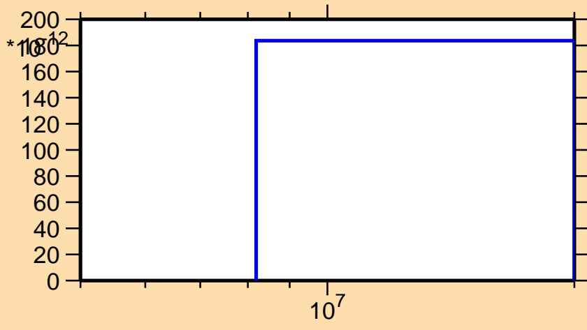
\sigma vs. E for ^{211}\text{Ra}(\text{mt117})
