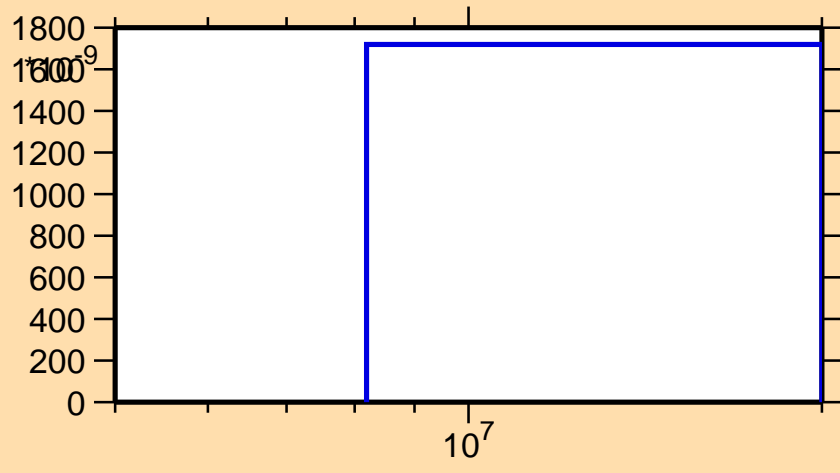
\sigma vs. E for ^{211}\text{Ra}(n,3n)
