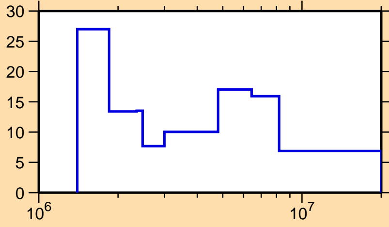
\Delta\sigma/\sigma vs. E for ^{211}\text{Ra}(n,\text{el.})
