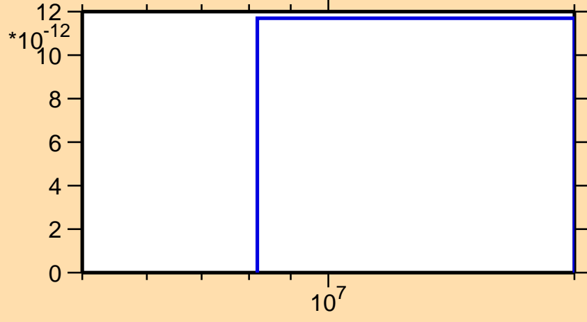
\sigma vs. E for ^{211}\text{Ra}(n,nt)
