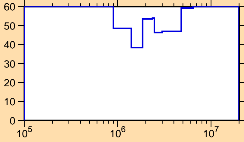
\Delta\sigma/\sigma vs. E for ^{211}\text{Ra}(n,n_1)
