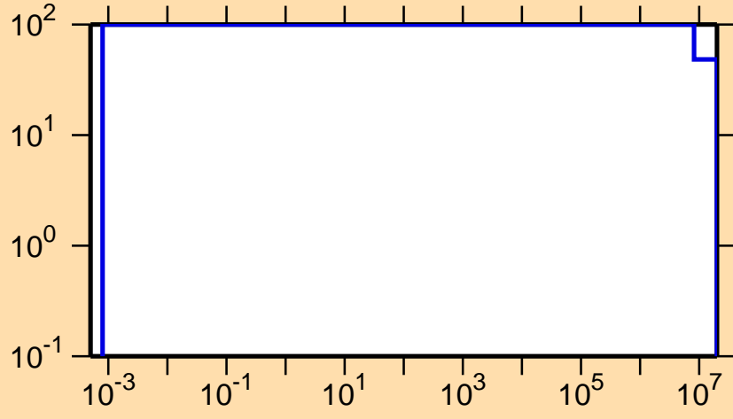
\Delta\sigma/\sigma vs. E for ^{211}\text{Ra}(n,p)
