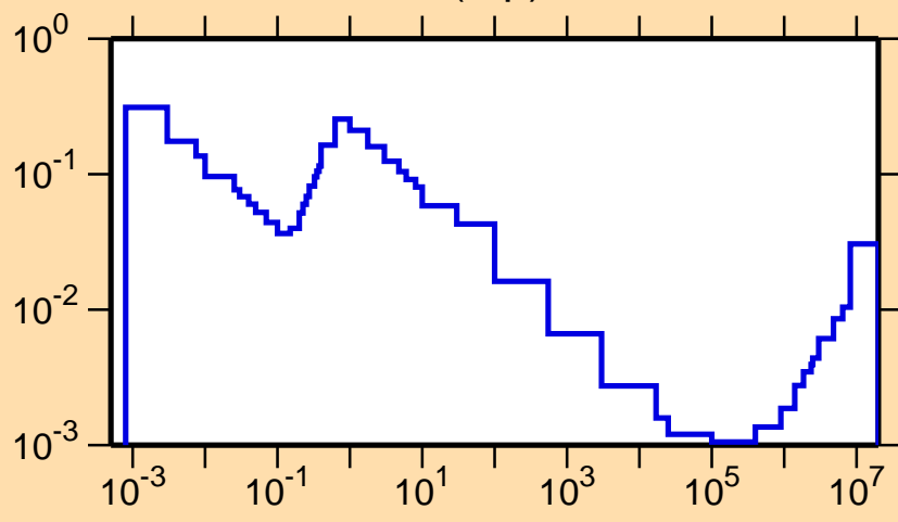
\sigma vs. E for ^{211}\text{Ra}(n,p)
