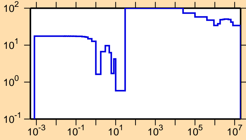
\Delta\sigma/\sigma vs. E for ^{211}\text{Ra}(n,\gamma)
