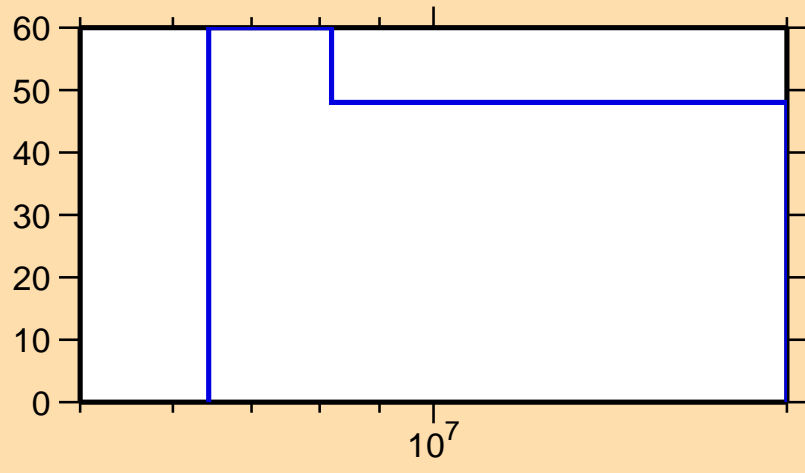
\Delta\sigma/\sigma vs. E for ^{211}\text{Ra}(n,2n)
