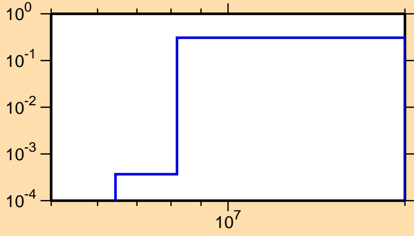
\sigma vs. E for ^{211}\text{Ra}(n,2n)
