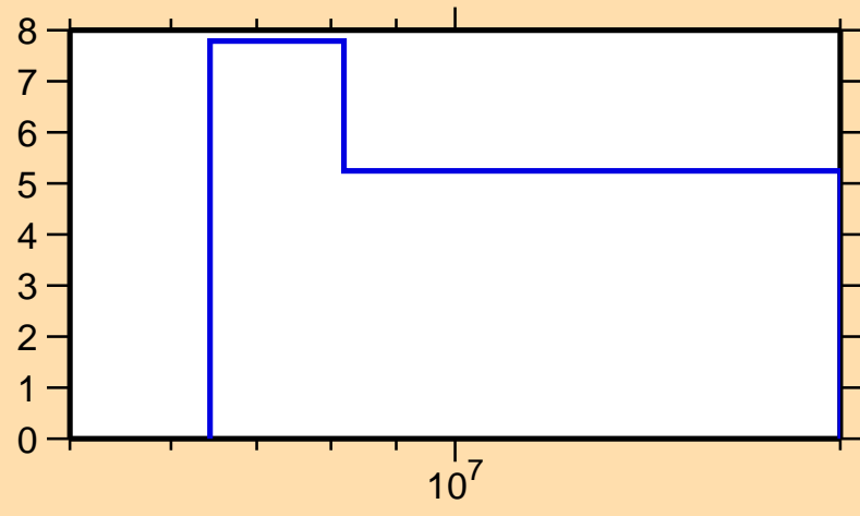
\Delta\sigma/\sigma vs. E for ^{211}\text{Ra}(n,\text{tot.})
