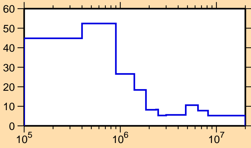
\Delta\sigma/\sigma vs. E for ^{211}\text{Ra}(n,\text{tot.})
