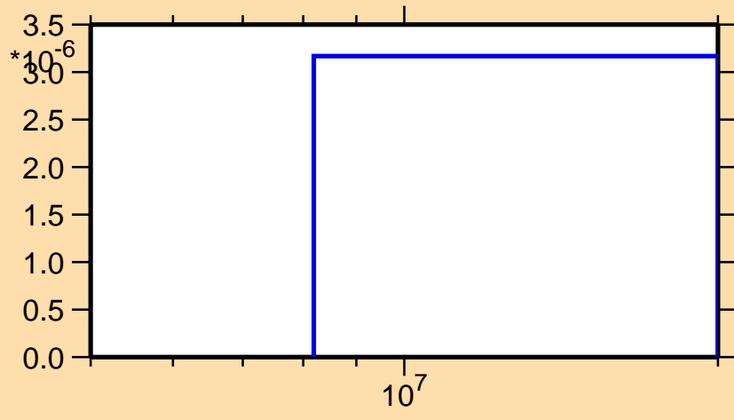
\sigma vs. E for ^{211}\text{Ra}(n,2np)
