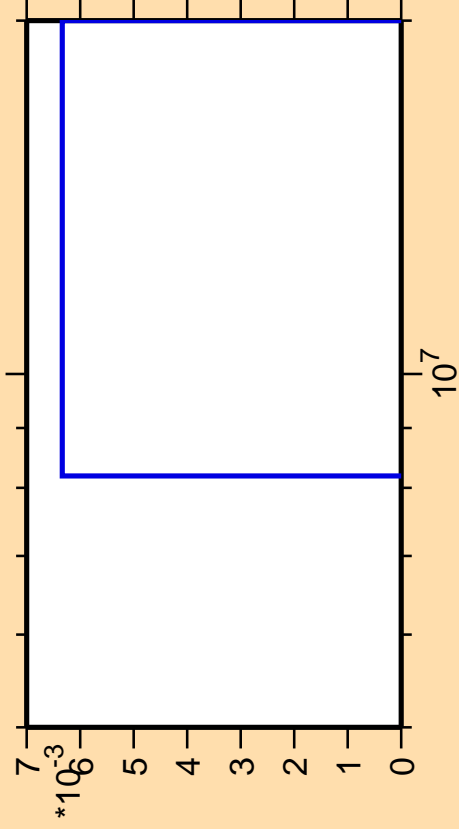
\Delta\sigma/\sigma vs. E for ^{211}\text{Ra}(n,3n\alpha)
