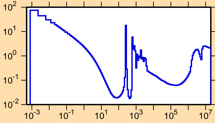
\sigma vs. E for ^{214}\text{Ra}(n,\text{nonel.})
