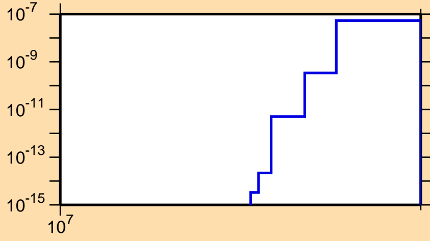
\sigma vs. E for ^{214}\text{Ra}(n,nt)
