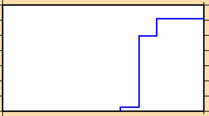
\sigma vs. E for ^{214}\text{Ra}(n,3n)
