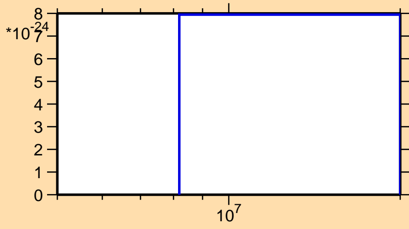
\sigma vs. E for ^{214}\text{Ra} (mt 42)
