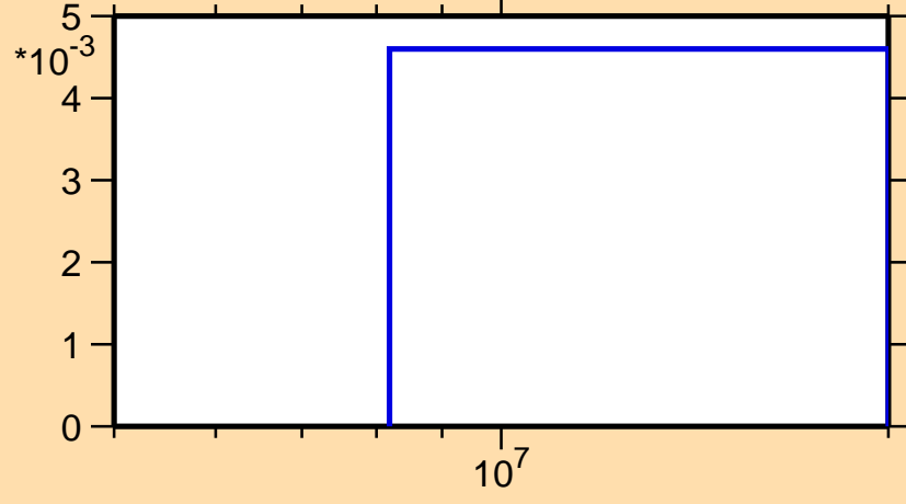
\sigma vs. E for ^{214}\text{Ra}(n,2n\alpha)
