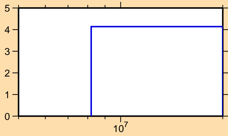
\Delta\sigma/\sigma vs. E for ^{214}\text{Ra}(n,\text{el.})
