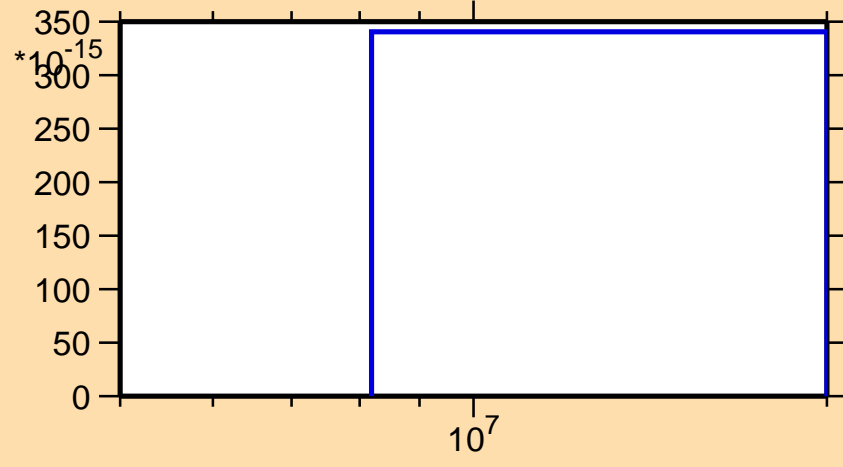
\sigma vs. E for ^{214}\text{Ra} (mt 34)
