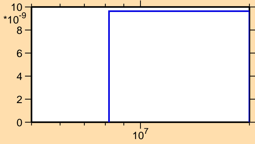
\sigma vs. E for ^{214}\text{Ra}(\text{mt117})
