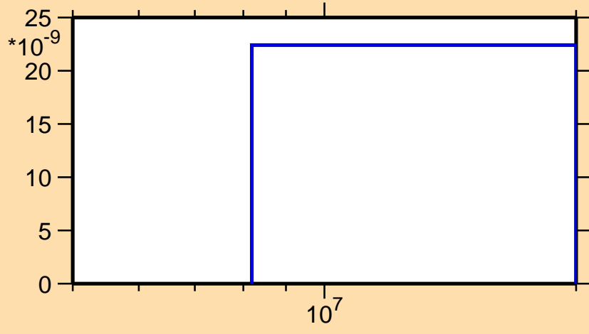
\sigma vs. E for ^{214}\text{Ra}(n,\text{He}3)
