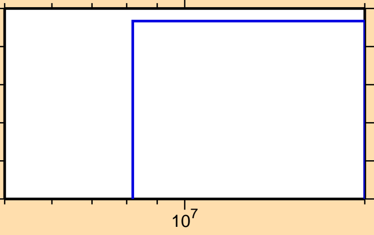
\sigma vs. E for ^{214}\text{Ra}(n,\text{nd})
