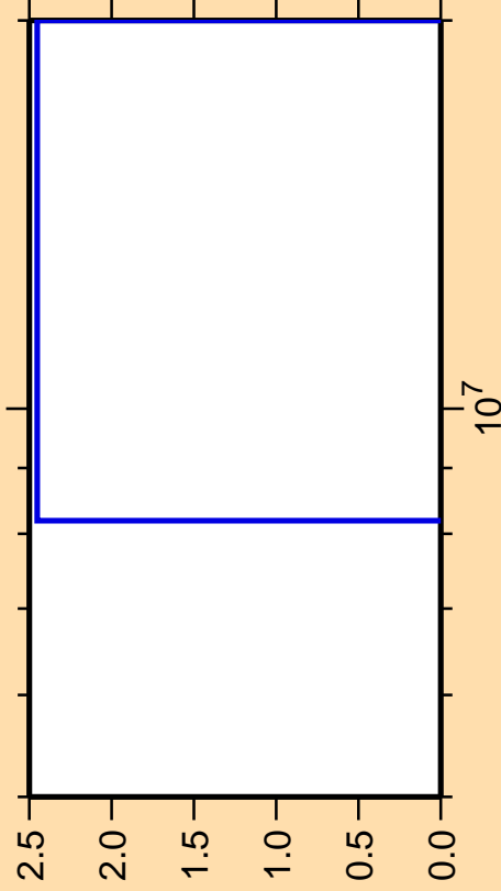
\Delta\sigma/\sigma vs. E for ^{214}\text{Ra} (mt 34)
