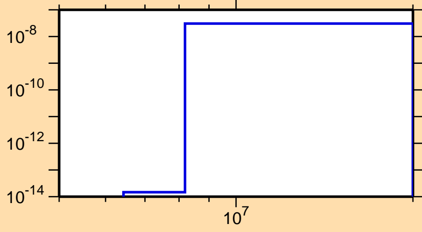
\sigma vs. E for ^{214}\text{Ra}(\text{mt } 45)
