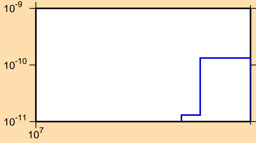
\sigma vs. E for ^{221}\text{Ra} (mt 45)
