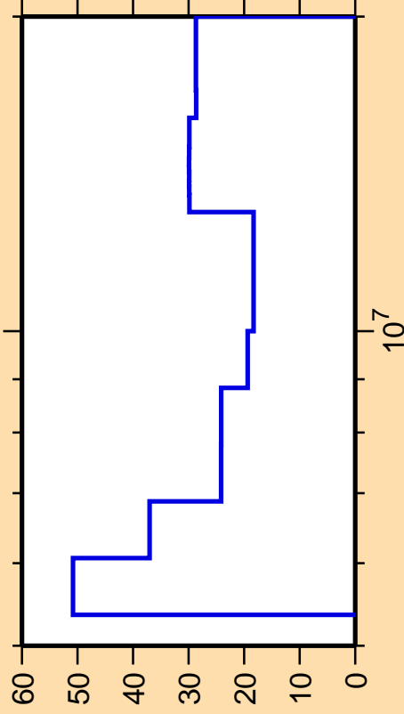
\Delta\sigma/\sigma vs. E for ^{221}\text{Ra}(n,2n)
