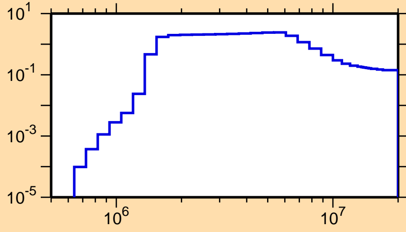
\sigma vs. E for ^{221}\text{Ra}(n,n\text{cont.})
