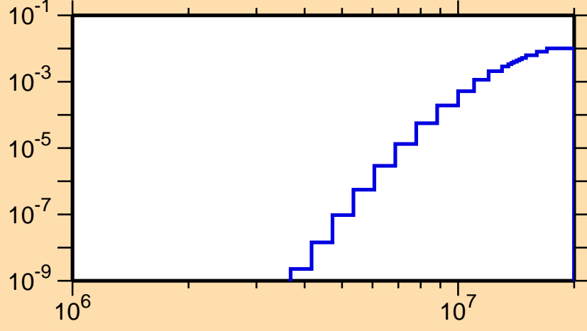
\sigma vs. E for ^{221}\text{Ra}(n,p)
