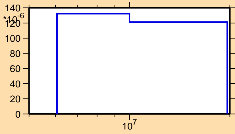
\sigma vs. E for ^{221}\text{Ra}(n,2n\alpha)
