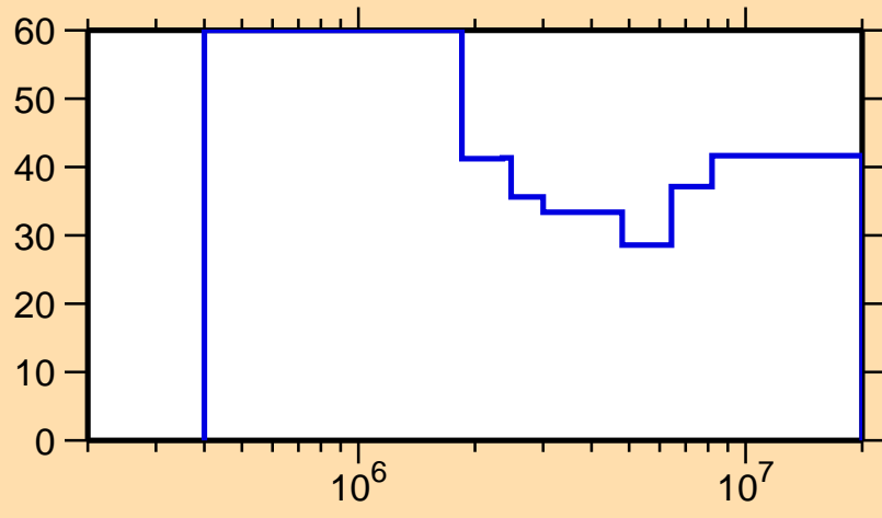
\Delta\sigma/\sigma vs. E for ^{221}\text{Ra}(n,n\text{cont.})
