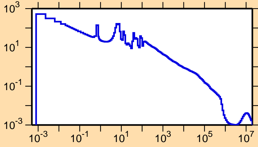
\sigma vs. E for ^{223}\text{Ra}(n,\gamma)
