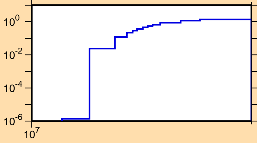
\sigma vs. E for ^{223}\text{Ra}(n,3n)
