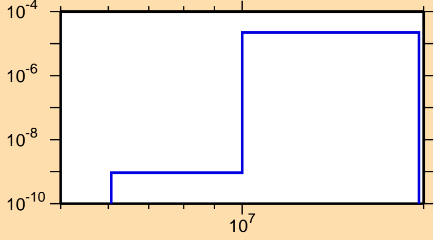
\sigma vs. E for ^{223}\text{Ra}(n,2n\alpha)
