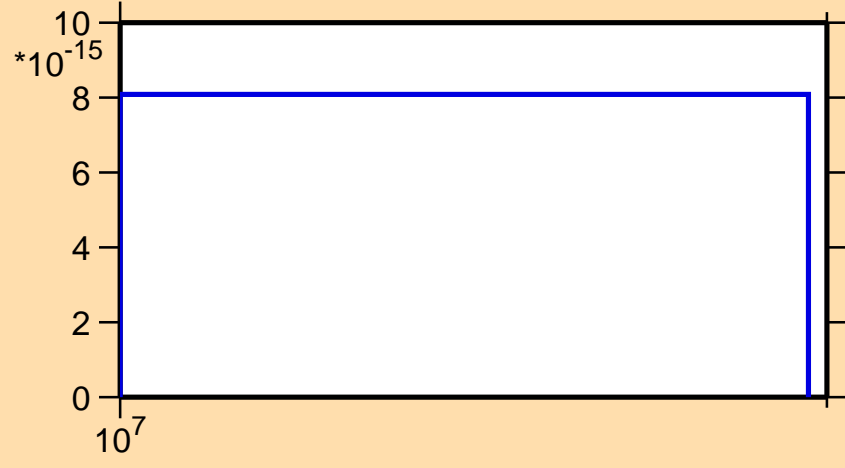
\sigma vs. E for ^{223}\text{Ra} (mt 34)
