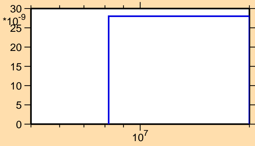
\sigma vs. E for ^{223}\text{Ra}(n,\text{nd})
