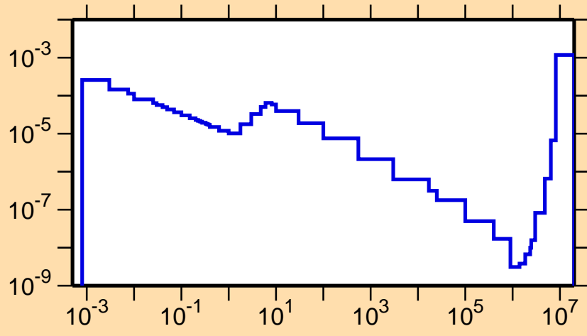
\sigma vs. E for ^{223}\text{Ra}(n,\alpha)
