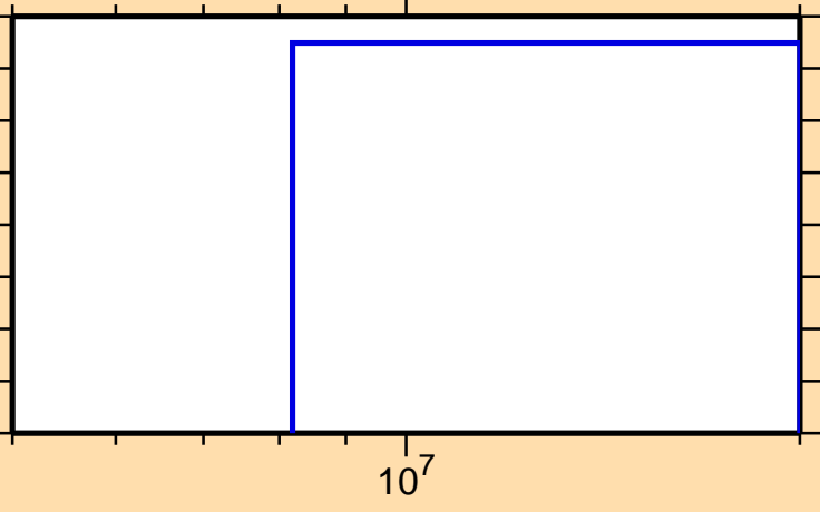
\sigma vs. E for ^{223}\text{Ra}(n,nt)
