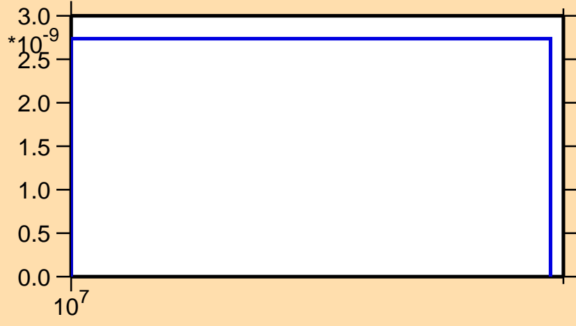
\sigma vs. E for ^{224}\text{Ra}(n,2np)
