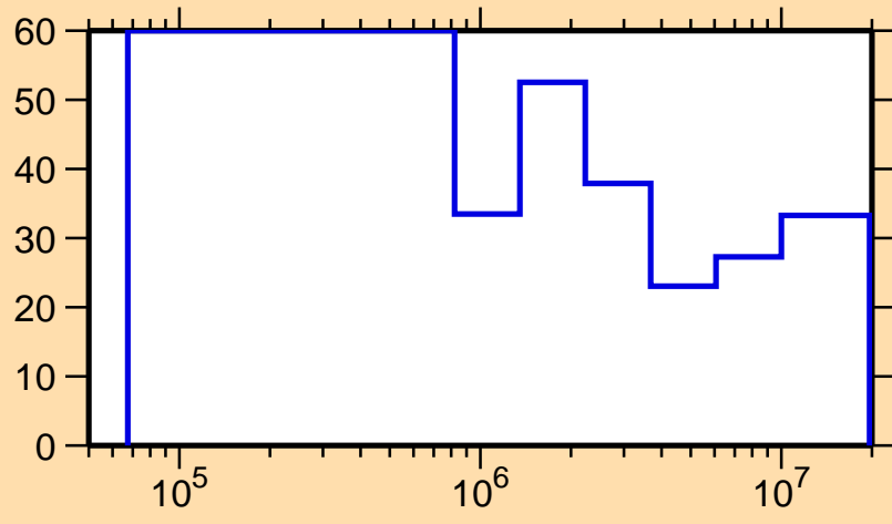
\Delta\sigma/\sigma vs. E for ^{224}\text{Ra}(n,n_1)
