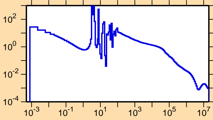
\sigma vs. E for ^{225}\text{Ra}(n,\gamma)
