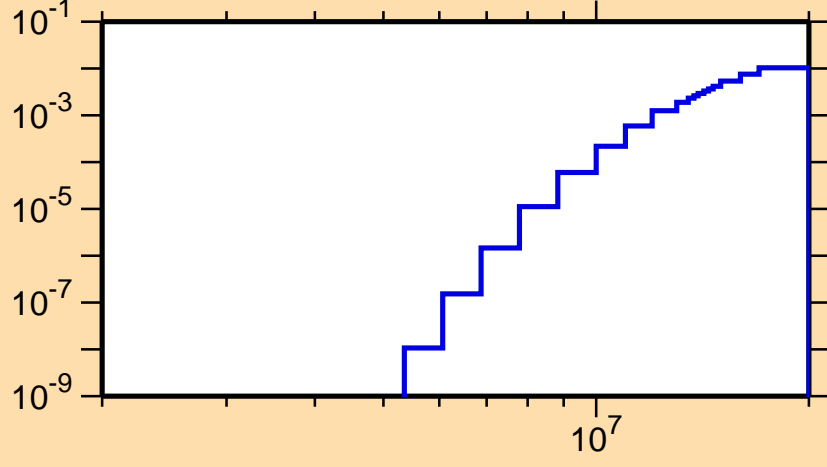
\sigma vs. E for ^{225}\text{Ra}(n,p)
