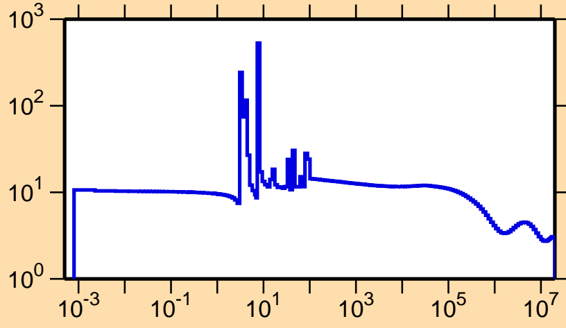
\sigma vs. E for ^{225}\text{Ra}(n,\text{el.})
