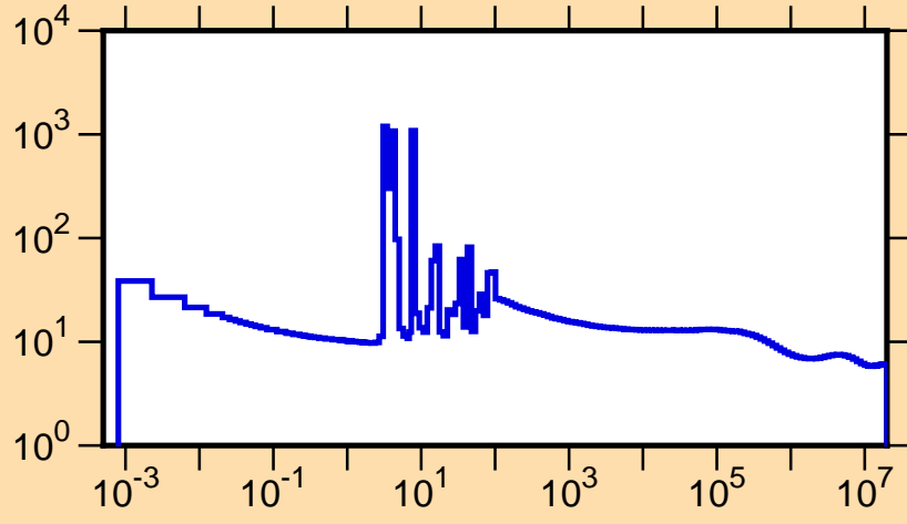
\sigma vs. E for ^{225}\text{Ra}(n,\text{tot.})
