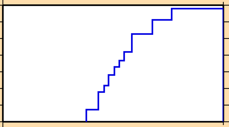
\sigma vs. E for ^{227}\text{Ra}(n,\text{nd})
