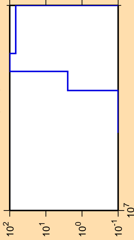
\Delta\sigma/\sigma vs. E for ^{227}\text{Ra}(n,nt)
