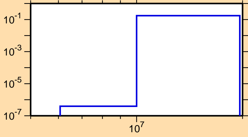
\sigma vs. E for ^{227}\text{Ra}(n,np)
