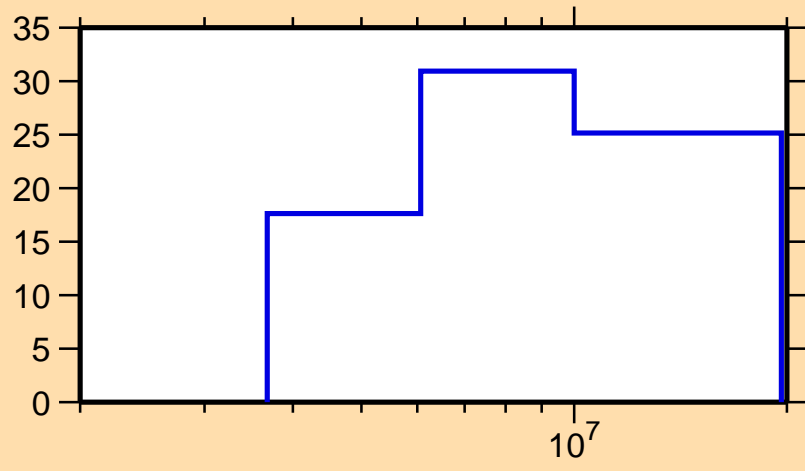
\Delta\sigma/\sigma vs. E for ^{227}\text{Ra}(n,\text{inel.})
