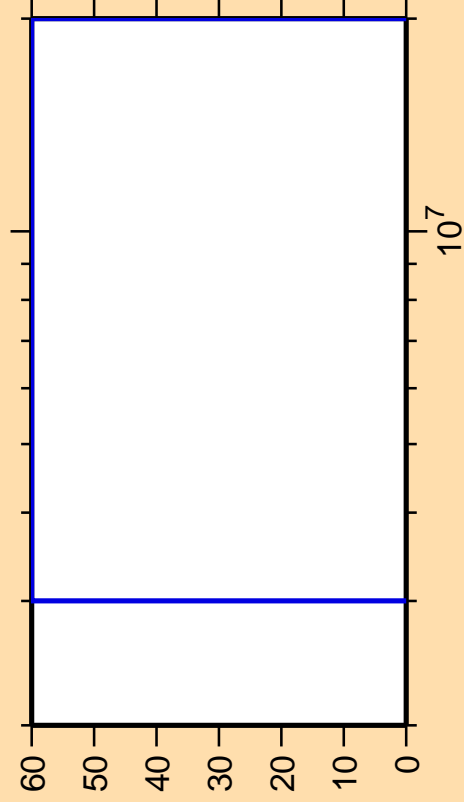
\Delta\sigma/\sigma vs. E for ^{227}\text{Ra}(n,\alpha)
