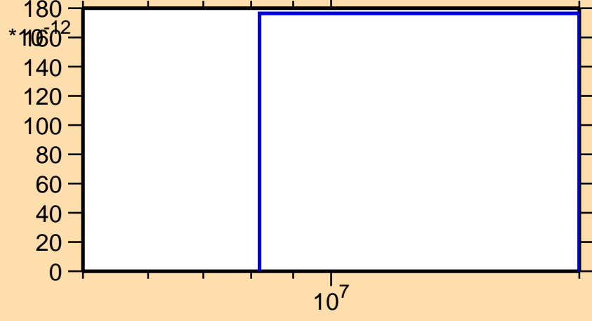
\sigma vs. E for ^{227}\text{Ra}(n,2n\alpha)
