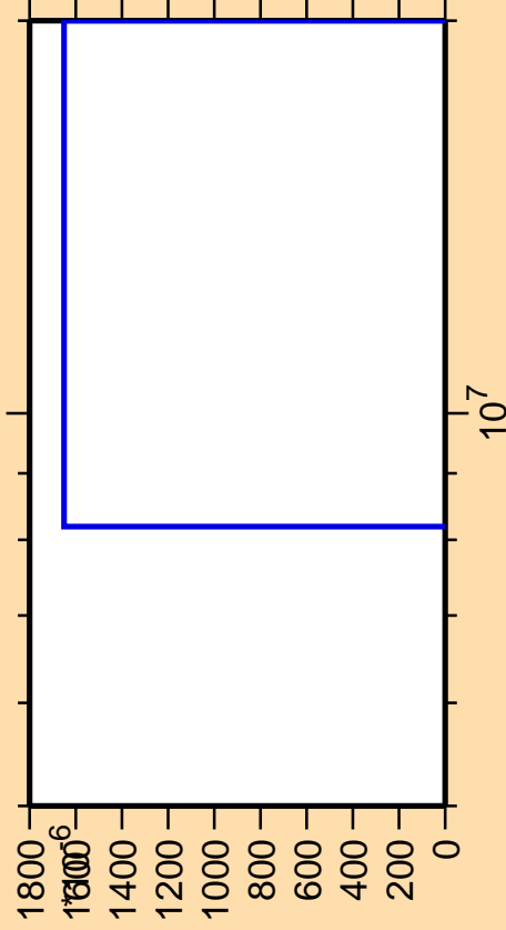
\Delta\sigma/\sigma vs. E for ^{227}\text{Ra}(n,3n\alpha)
