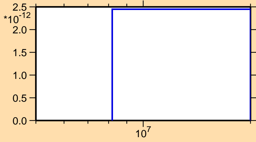
\sigma vs. E for ^{227}\text{Ra}(n,2np)
