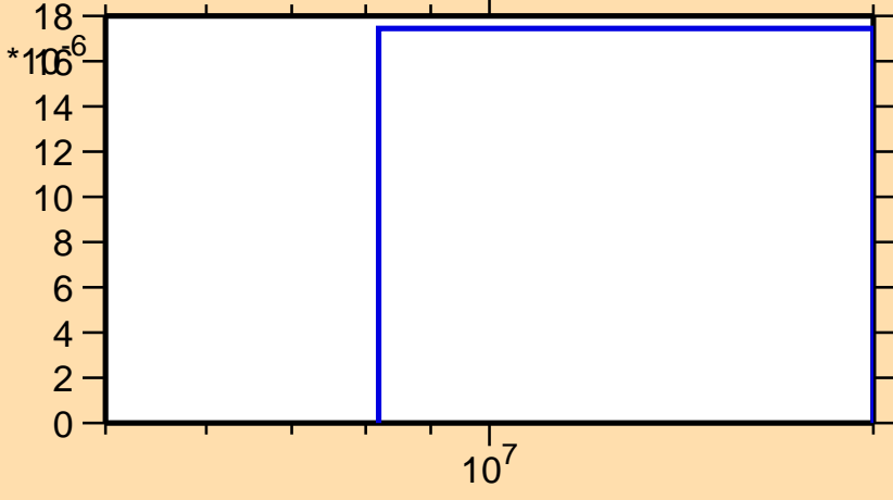
\sigma vs. E for ^{227}\text{Ra}(n,t)
