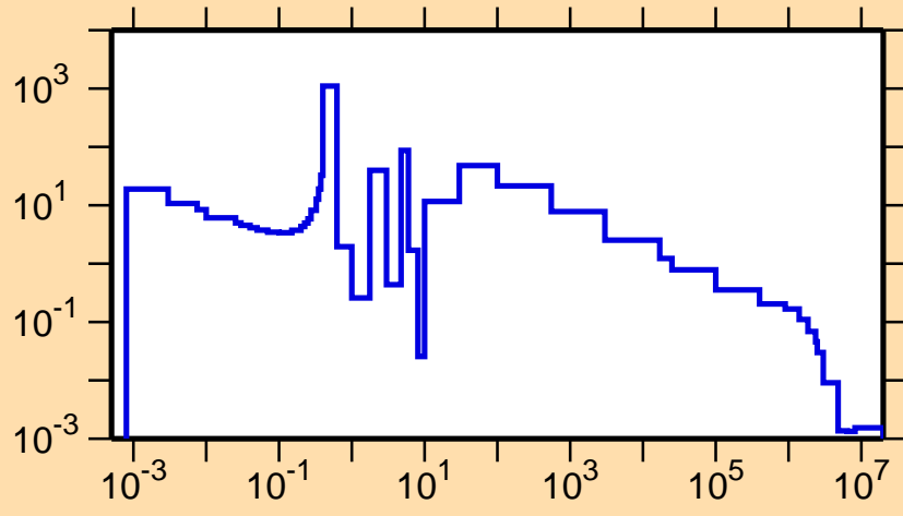
\sigma vs. E for ^{227}\text{Ra}(n,\gamma)
