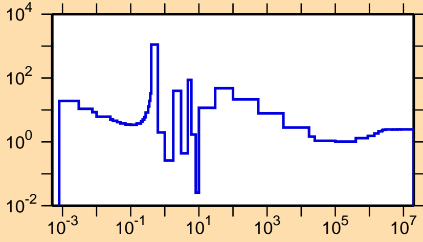
\sigma vs. E for ^{227}\text{Ra}(n,\text{nonel.})
