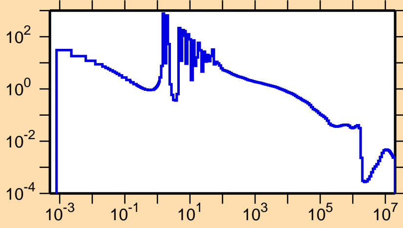
\sigma vs. E for ^{229}\text{Ra}(n,\gamma)
