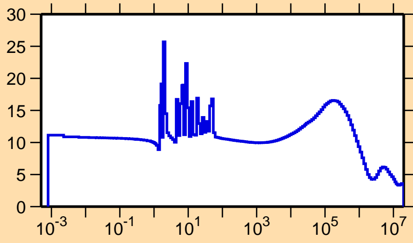
\sigma vs. E for ^{229}\text{Ra}(n,\text{el.})
