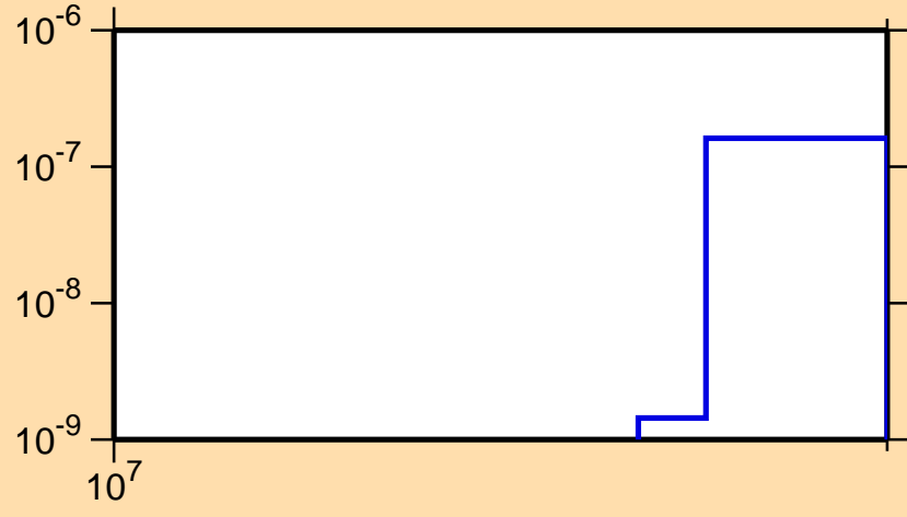
\sigma vs. E for ^{229}\text{Ra}(n,2np)
