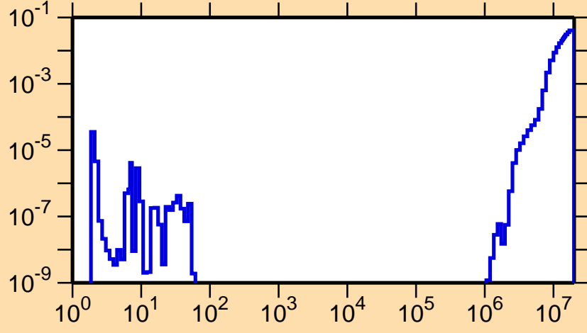
\sigma vs. E for ^{229}\text{Ra}(n,f)
