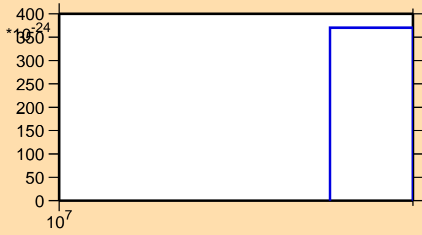
\sigma vs. E for ^{229}\text{Ra} (mt 42)
