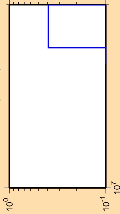
\Delta\sigma/\sigma vs. E for ^{229}\text{Ra}(n,\text{He3})
