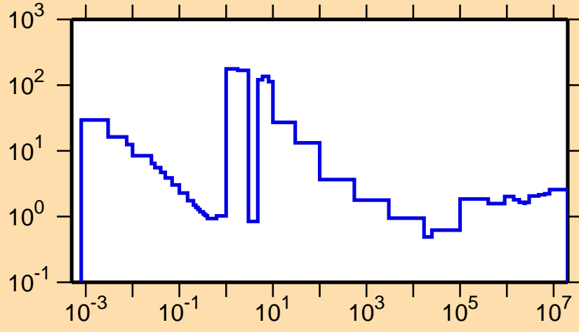
\sigma vs. E for ^{229}\text{Ra}(n,\text{nonel.})
