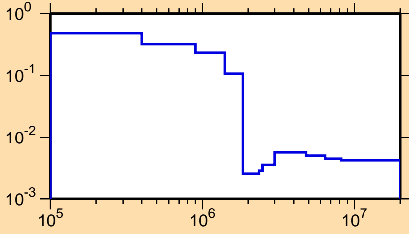
\sigma vs. E for ^{229}\text{Ra}(n,n_2)
