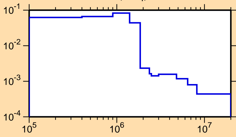
\sigma vs. E for ^{229}\text{Ra}(n,n_4)
