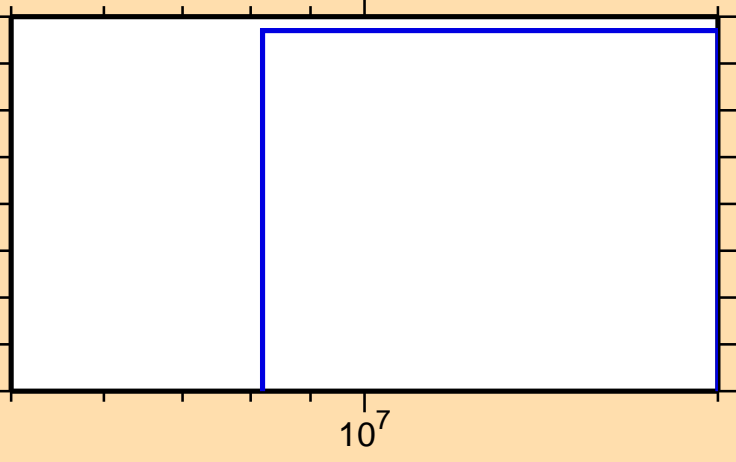
\sigma vs. E for ^{229}\text{Ra}(n,3n)
