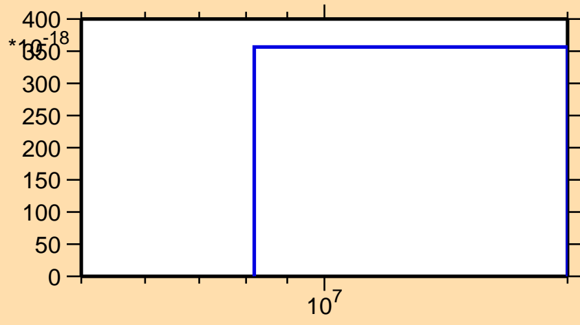
\sigma vs. E for ^{229}\text{Ra}(n,\text{He}3)
