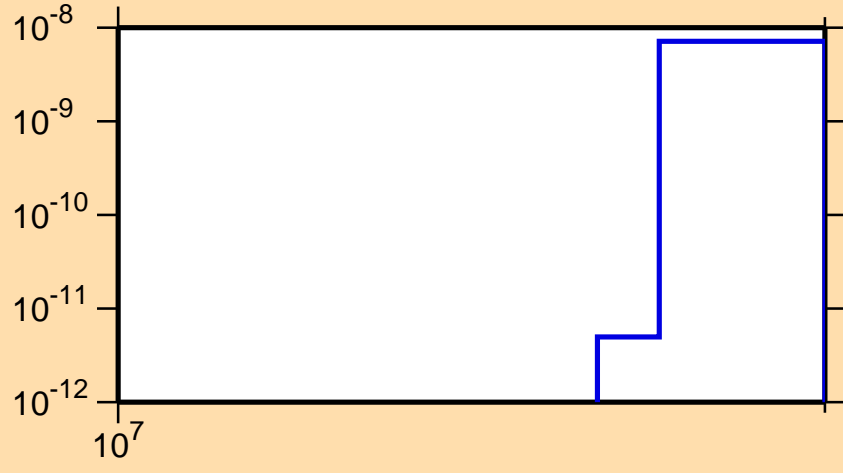
\sigma vs. E for ^{231}\text{Ra}(n,2np)
