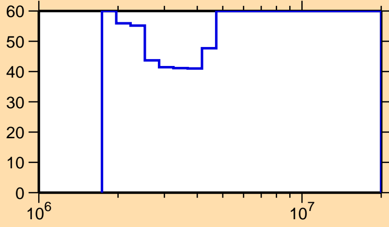
\Delta\sigma/\sigma vs. E for ^{231}\text{Ra}(n,n\text{cont.})
