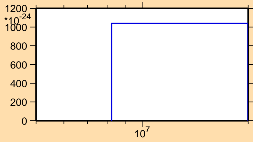
\sigma vs. E for ^{231}\text{Ra} (mt 42)
