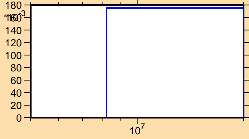
\sigma vs. E for ^{231}\text{Ra}(n,3n)
