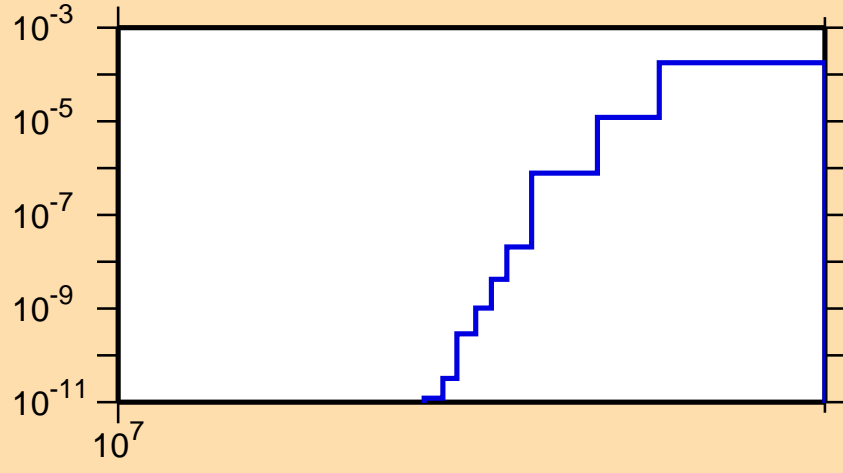
\sigma vs. E for ^{232}\text{Ra}(n,nt)
