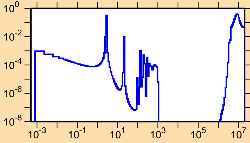
\sigma vs. E for ^{232}\text{Ra}(n,f)
