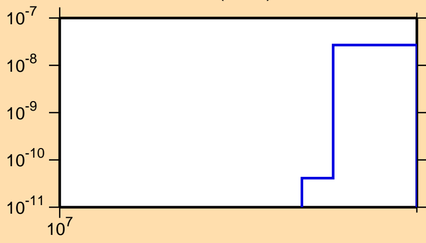
\sigma vs. E for ^{232}\text{Ra}(n,\text{nd})
