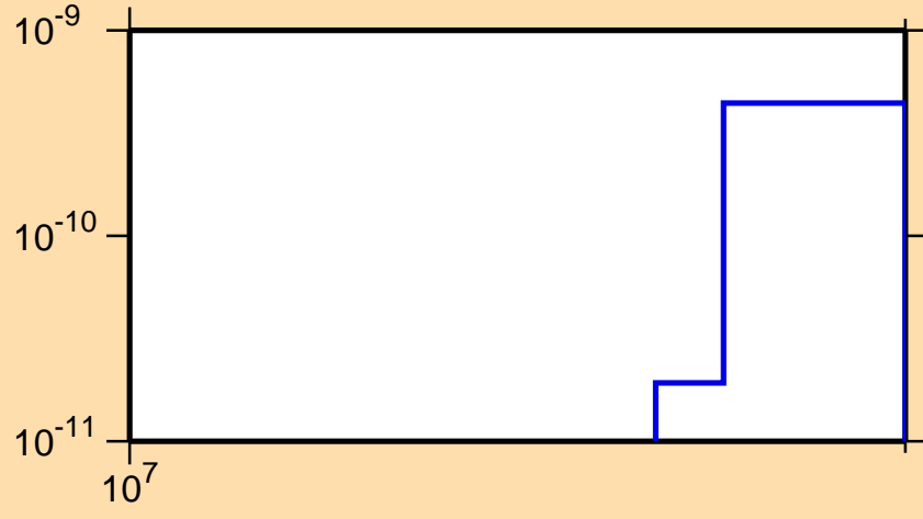
\sigma vs. E for ^{232}\text{Ra}(n,3n\alpha)
