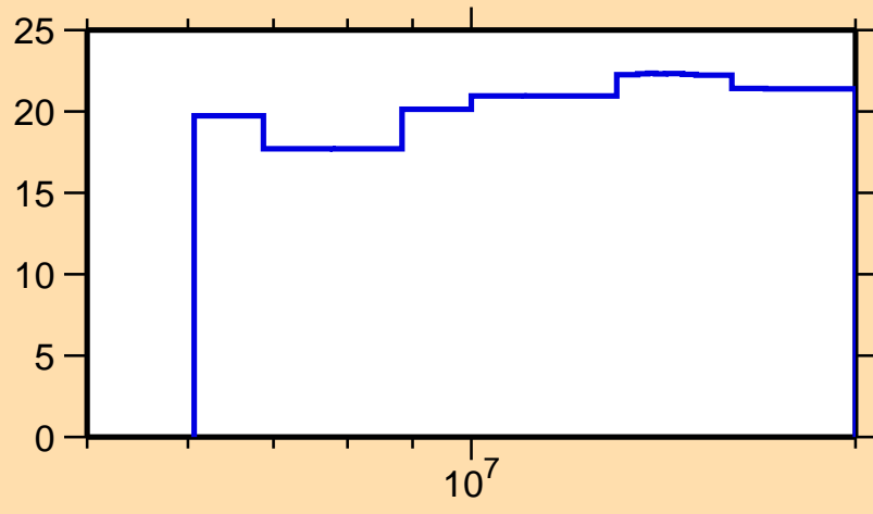
\Delta\sigma/\sigma vs. E for ^{232}\text{Ra}(n,\text{nonel.})
