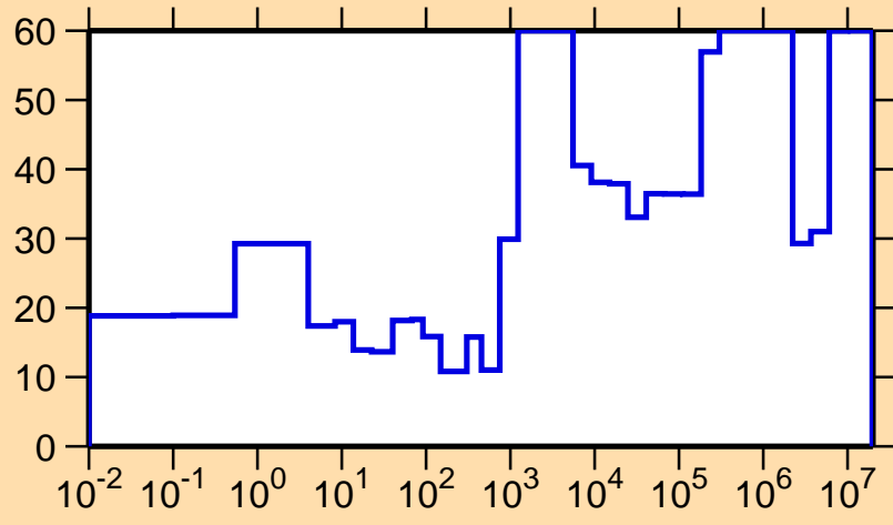
\Delta\sigma/\sigma vs. E for ^{232}\text{Ra}(n,el.)
