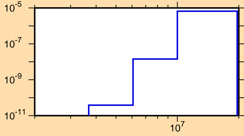
\sigma vs. E for ^{232}\text{Ra}(n,\alpha)
