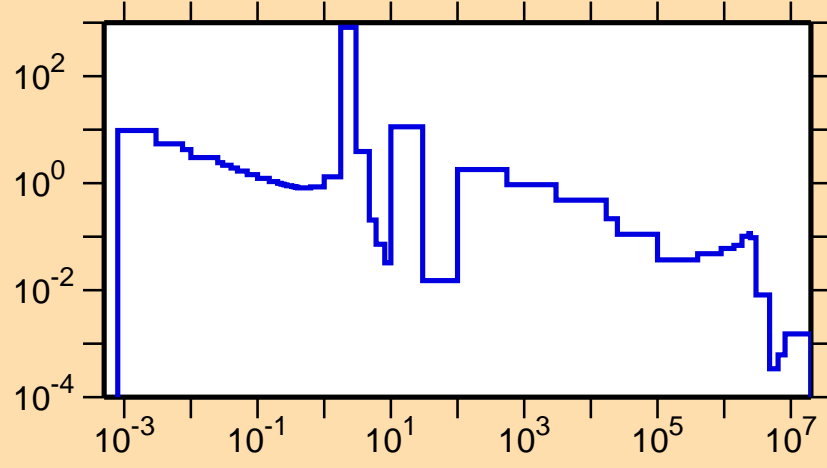
\sigma vs. E for ^{232}\text{Ra}(n,\gamma)
