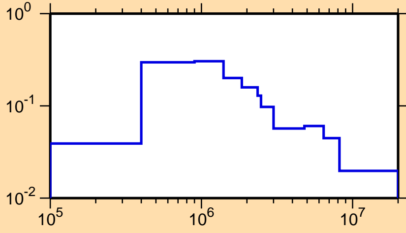
\sigma vs. E for ^{232}\text{Ra}(n,n_2)
