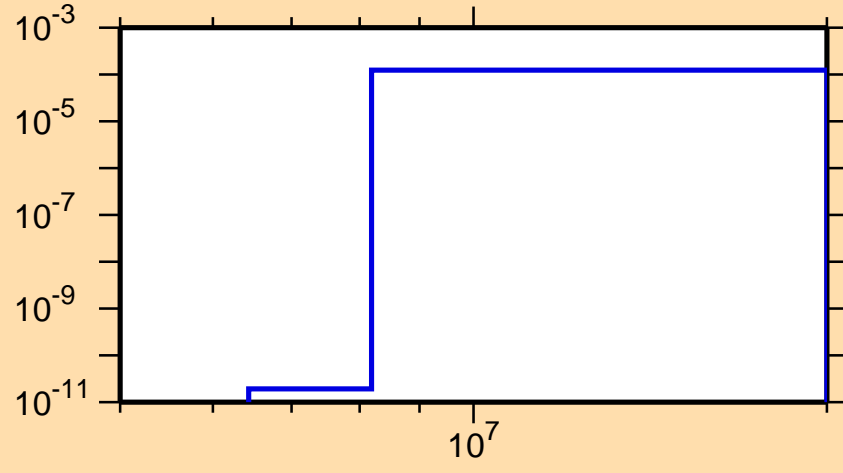
\sigma vs. E for ^{232}\text{Ra}(n,n\alpha)
