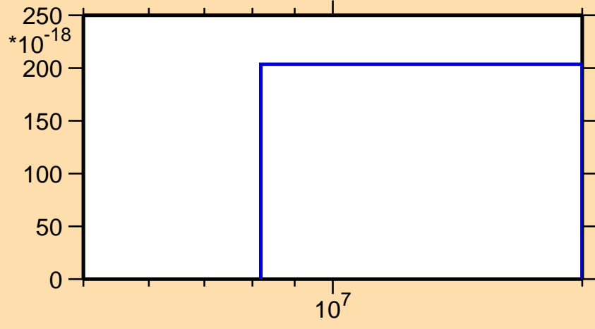
\sigma vs. E for ^{232}\text{Ra} (mt 42)
