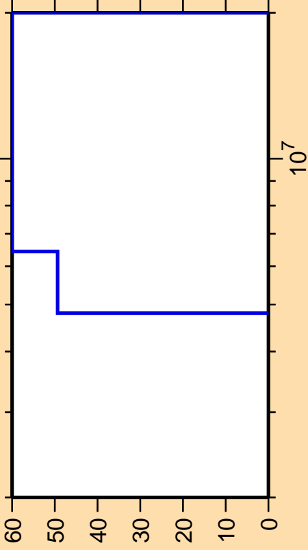
\Delta\sigma/\sigma vs. E for ^{232}\text{Ra}(n,n\text{cont.})
