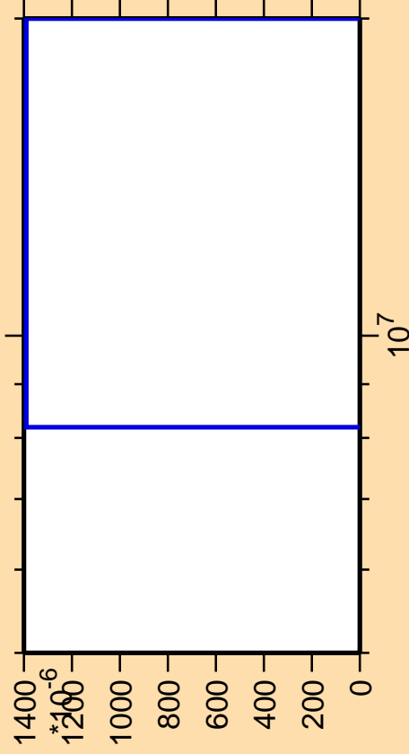
\Delta\sigma/\sigma vs. E for ^{232}\text{Ra} (mt 42)
