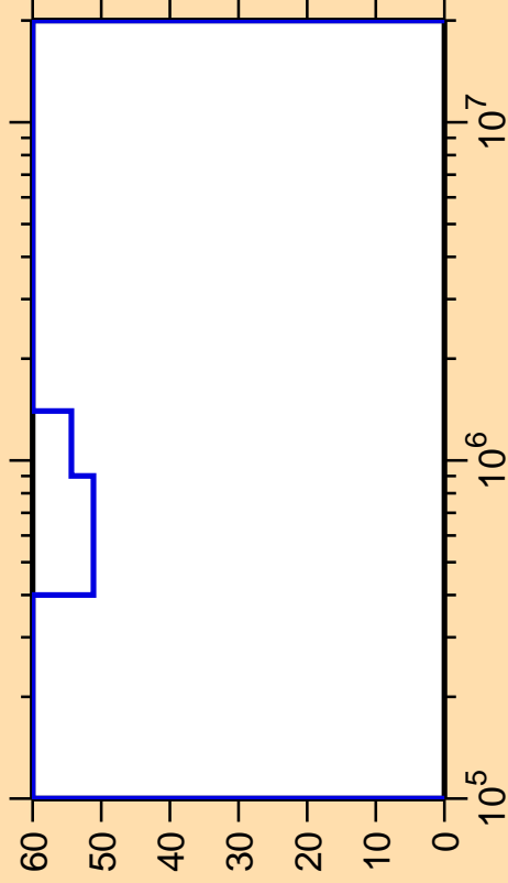
\Delta\sigma/\sigma vs. E for ^{232}\text{Ra}(n,n_2)
