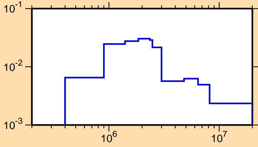
\sigma vs. E for ^{232}\text{Ra}(n,n_3)
