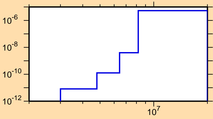
\sigma vs. E for ^{232}\text{Ra}(n,\alpha)
