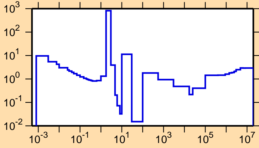
\sigma vs. E for ^{232}\text{Ra}(n,\text{nonel.})
