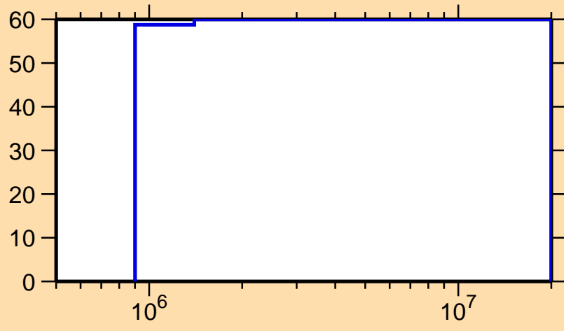
\Delta\sigma/\sigma vs. E for ^{232}\text{Ra}(n,n_1)
