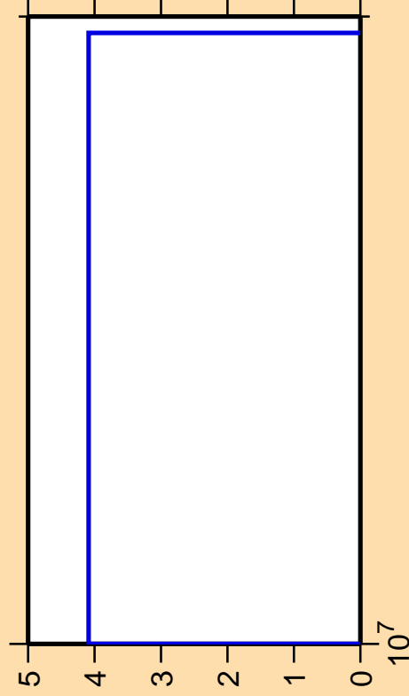
\Delta\sigma/\sigma vs. E for ^{233}\text{Ra}(n,3n\alpha)
