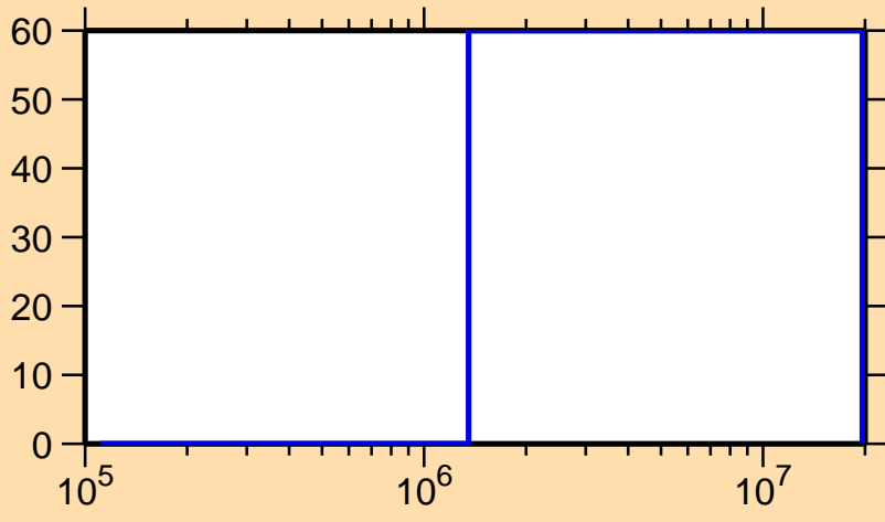
\Delta\sigma/\sigma vs. E for ^{233}\text{Ra}(n,f)
