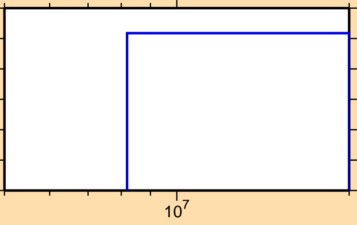
\sigma vs. E for ^{233}\text{Ra}(n,2np)
