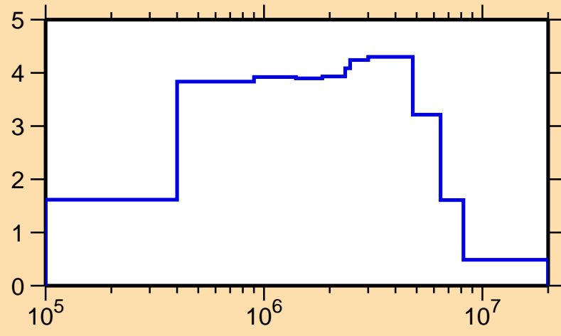
\sigma vs. E for ^{233}\text{Ra}(n,\text{inel.})
