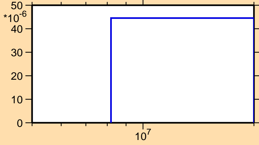
\sigma vs. E for ^{233}\text{Ra}(n,n\alpha)
