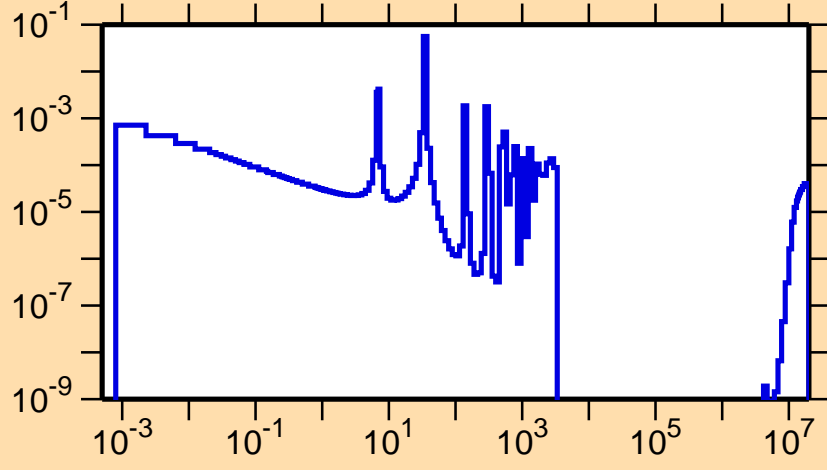
\sigma vs. E for ^{234}\text{Ra}(n,f)
