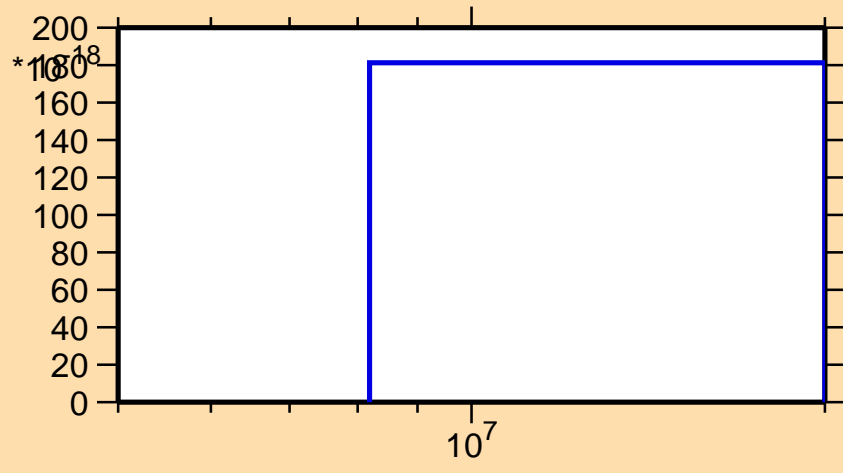
\sigma vs. E for ^{234}\text{Ra}(n,3n\alpha)
