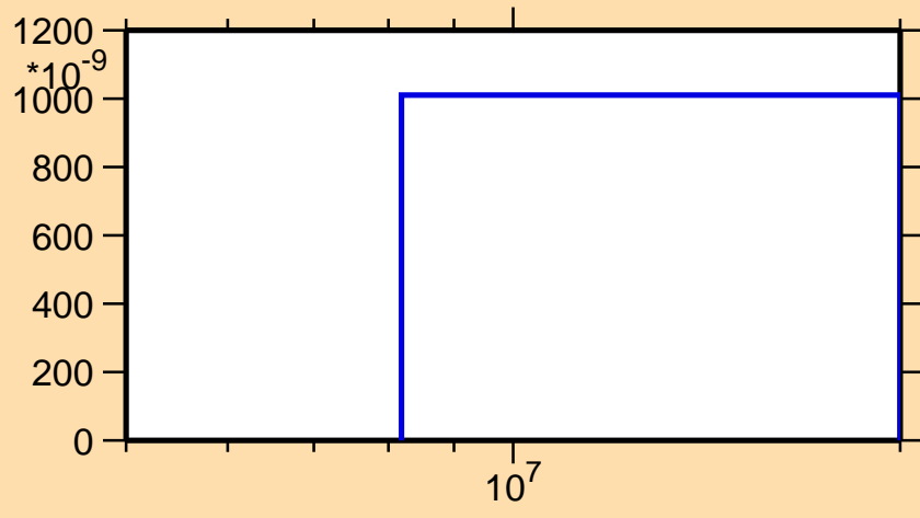
\sigma vs. E for ^{234}\text{Ra}(n,d)
