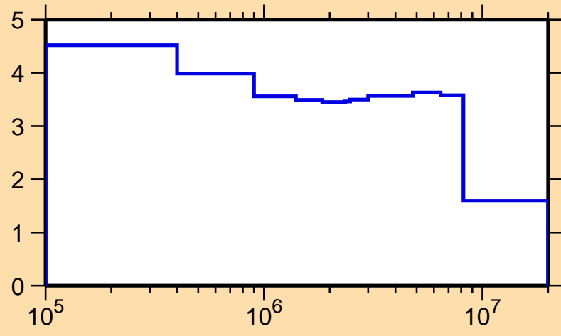
\sigma vs. E for ^{234}\text{Ra}(n,n\text{cont.})
