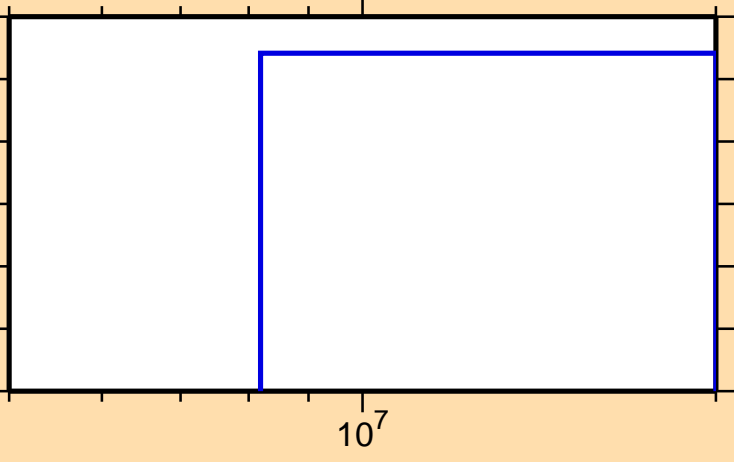
\sigma vs. E for ^{234}\text{Ra}(n,t)
