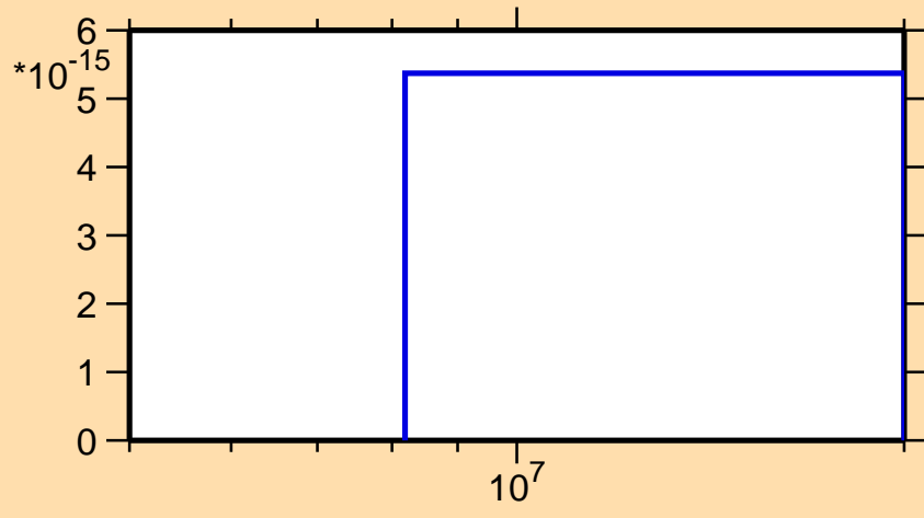
\sigma vs. E for ^{234}\text{Ra}(n,\text{nd})
