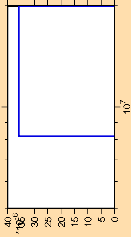
\Delta\sigma/\sigma vs. E for ^{234}\text{Ra}(n,2np)
