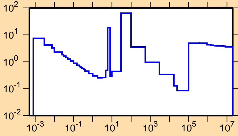
\sigma vs. E for ^{234}\text{Ra}(n,\text{nonel.})
