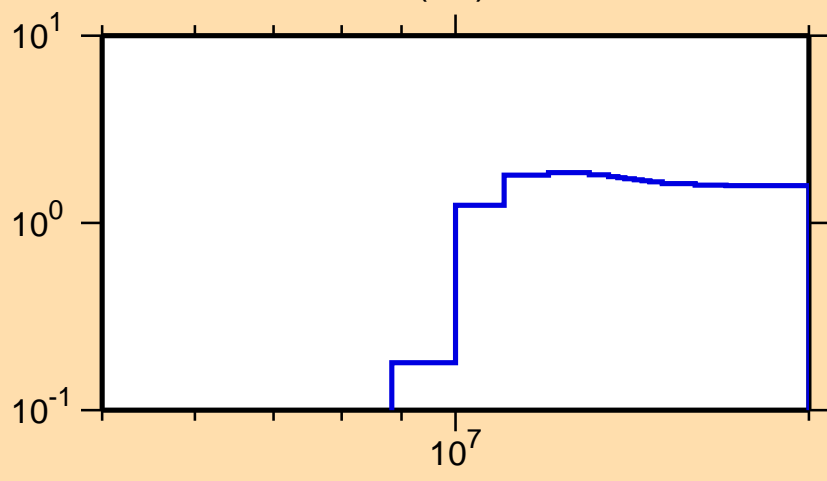
\sigma vs. E for ^{235}\text{Ra}(n,t)
