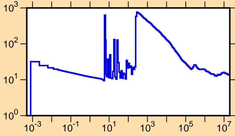
\sigma vs. E for ^{235}\text{Ra}(n,\text{tot.})
